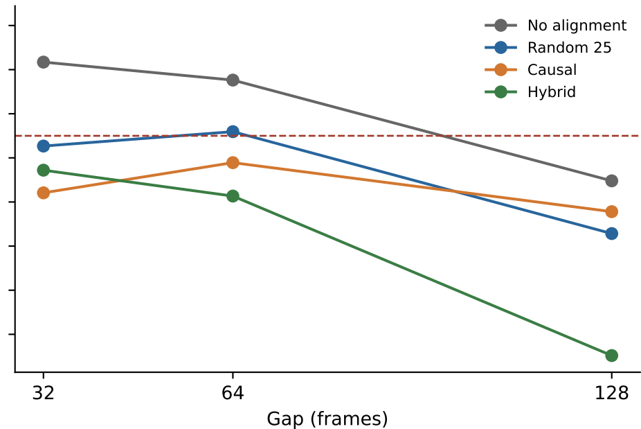
PointMaze
