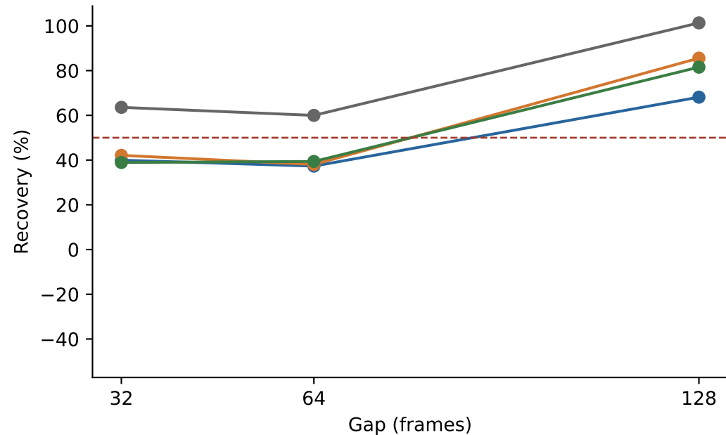
Cube
