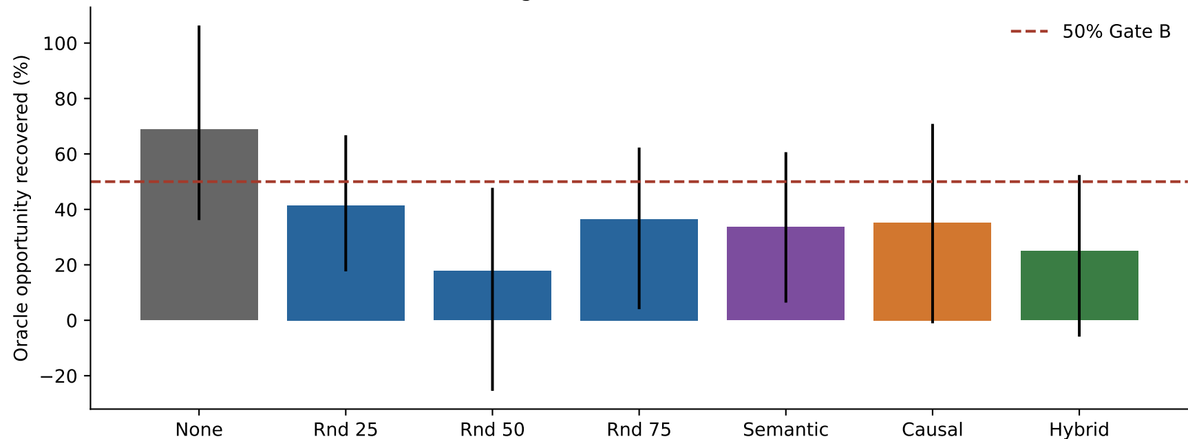
Patch alignment factorial · six full cells
