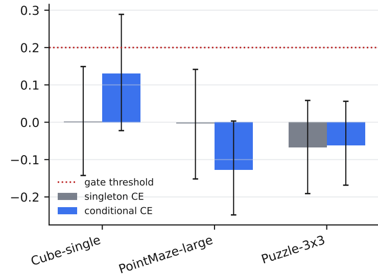
Within-query Spearman
