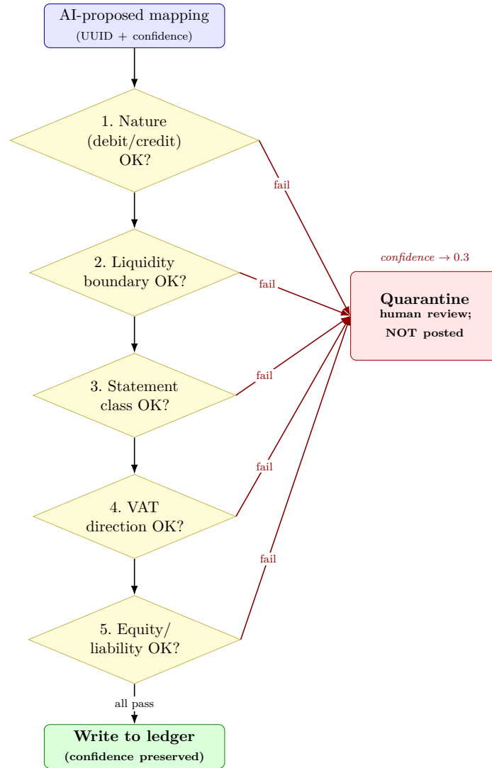
Figure 7: The Deterministic Boundary Library as a validation gauntlet. An AI-proposed mapping must satisfy a sequence of deterministic accounting invariants — the five exercised in the validation harness (nature, liquidity, statement class, VAT direction, and equity/liability classification). Any single failure quarantines the proposal for human review with a penalised confidence score; it is not posted to the ledger. Only a clean pass on every invariant reaches the ledger write path.
