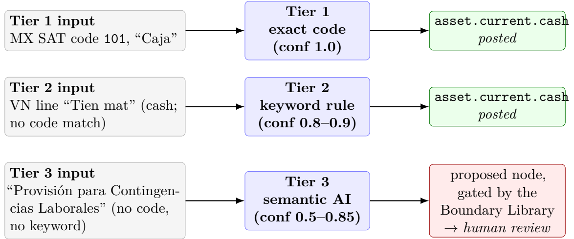
Figure 6: The three tiers on concrete inputs. Tier 1 resolves a statutory code deterministically; Tier 2 resolves a name via an auditable multilingual rule when no code matches; Tier 3 (the only stochastic step) proposes a node when neither deterministic tier fires, and that proposal is constrained to existing universal nodes and gated by the Deterministic Boundary Library before it can post. The engine descends the tiers only on failure, so most volume resolves at Tier 1-2 without inference.
