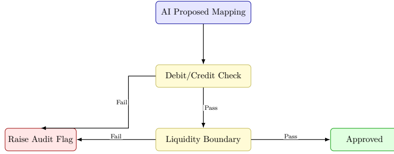
Figure 6: The deterministic boundary checklist verifies AI-proposed mappings prior to ledger write-in.
