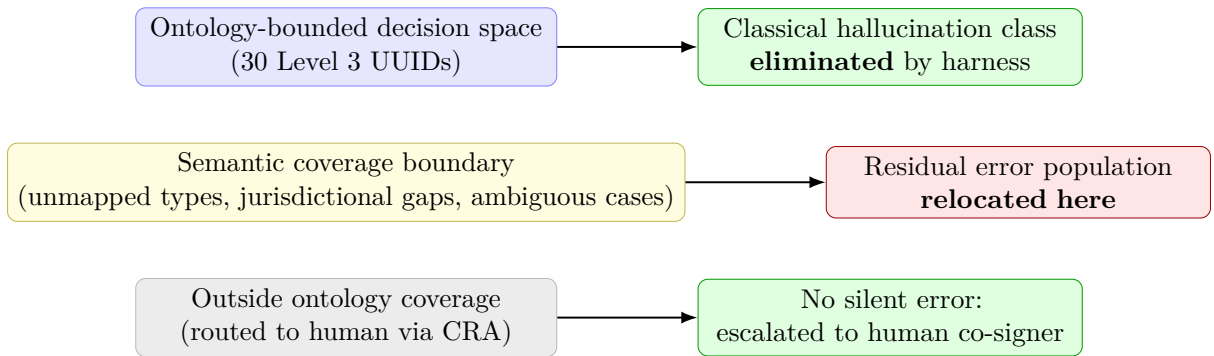
Figure 7: Locus of error before and after ontology-as-constraint is applied. Classical hallucination (arbitrary invalid outputs) is eliminated at the harness layer. Residual errors relocate to the semantic coverage boundary: unmapped transaction types, incomplete jurisdictional rules, and semantically ambiguous cases within valid UUID space. Cases outside coverage are escalated to human review rather than silently committed.
