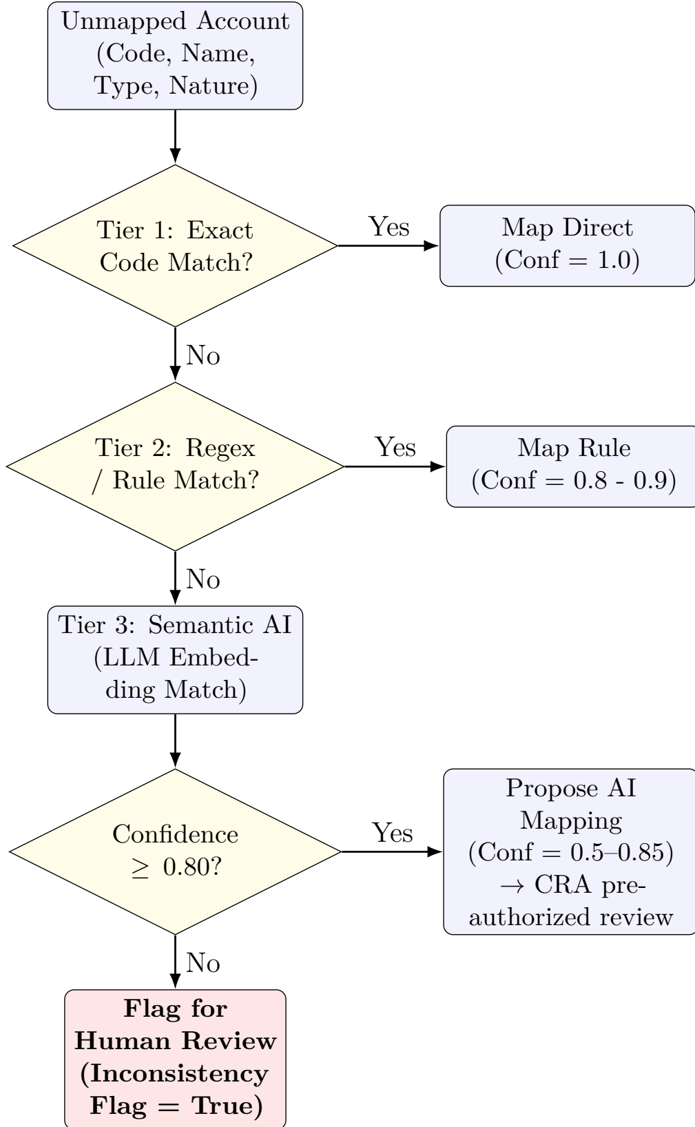
Figure 5: The Three-Tier Resolution Pipeline. Local ERP accounts pass through exact code checks (Tier 1) and rule-based regex parsing (Tier 2) before falling back to Semantic AI (Tier 3). All outputs enter the Co-responsibility Architecture (CRA): high-confidence proposals ( \geq 0.80 ) are queued for pre-authorized review with audit logging; low-confidence or boundary-violating proposals require explicit human co-signature before ledger write-in. In no case does the agent commit a mapping to the ledger without a human-authorized or human-pre-authorized pathway.
