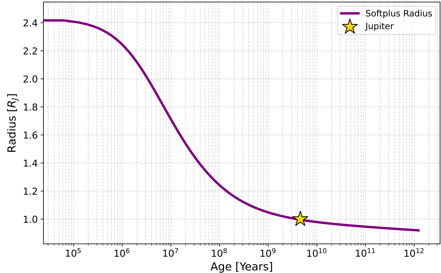
Structural Evolution (Softplus)
