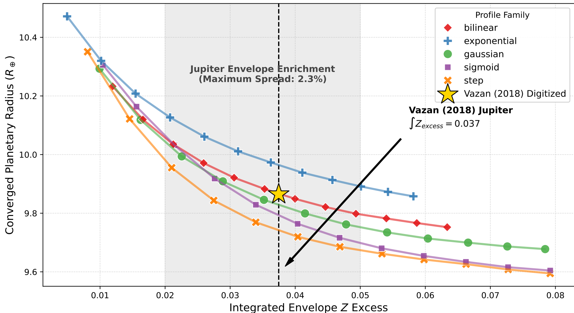
Radius Robustness to Functional Form ( Z_{base} = 0.081, Z_{core} = 0.240 )
