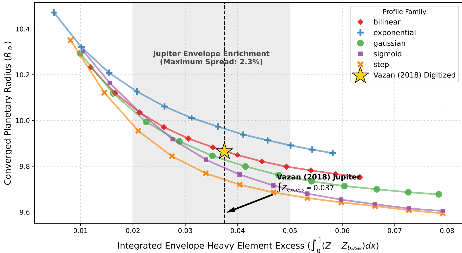
Radius Robustness to Functional Form ( T_{surf} = 165 \text{ K} , M_{core} = 0.1 M_{\oplus} )
