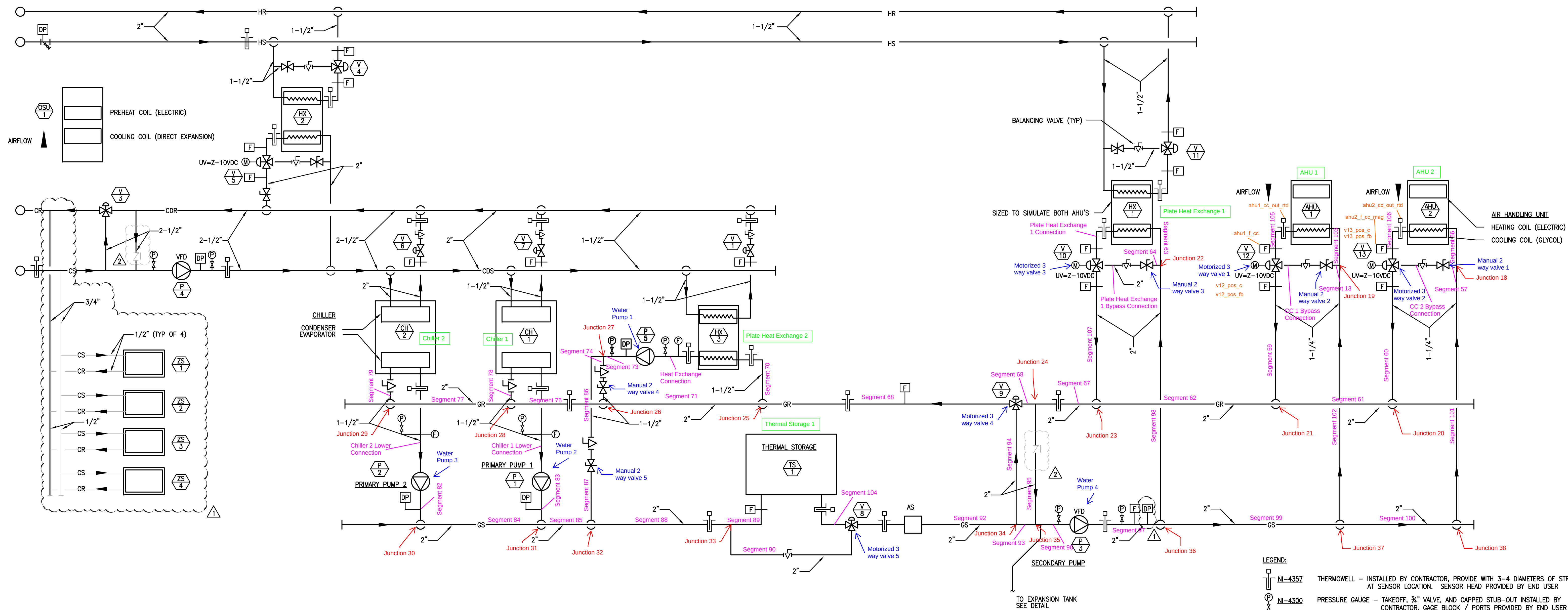
2 HYDRONIC DIAGRAM NOT TO SCALE
