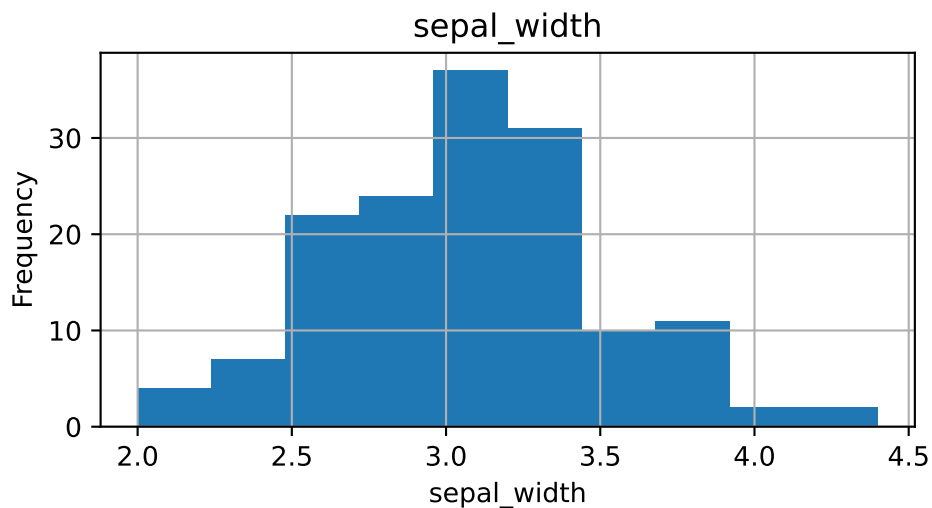
Figure 1: Distribution of Numerical Features
