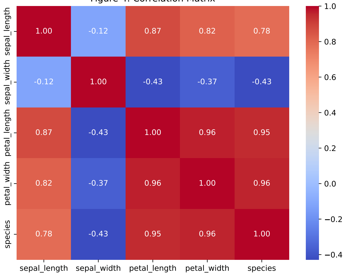
Figure 4: Correlation Matrix
