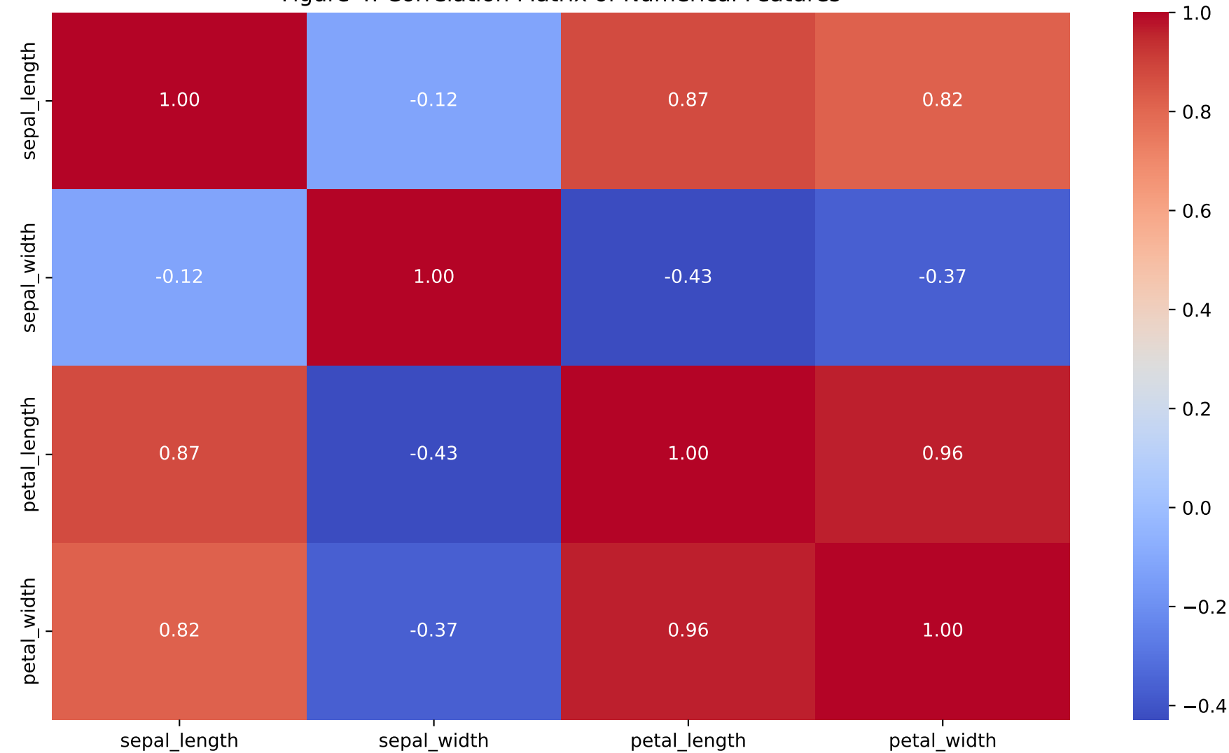
Figure 4: Correlation Matrix of Numerical Features
