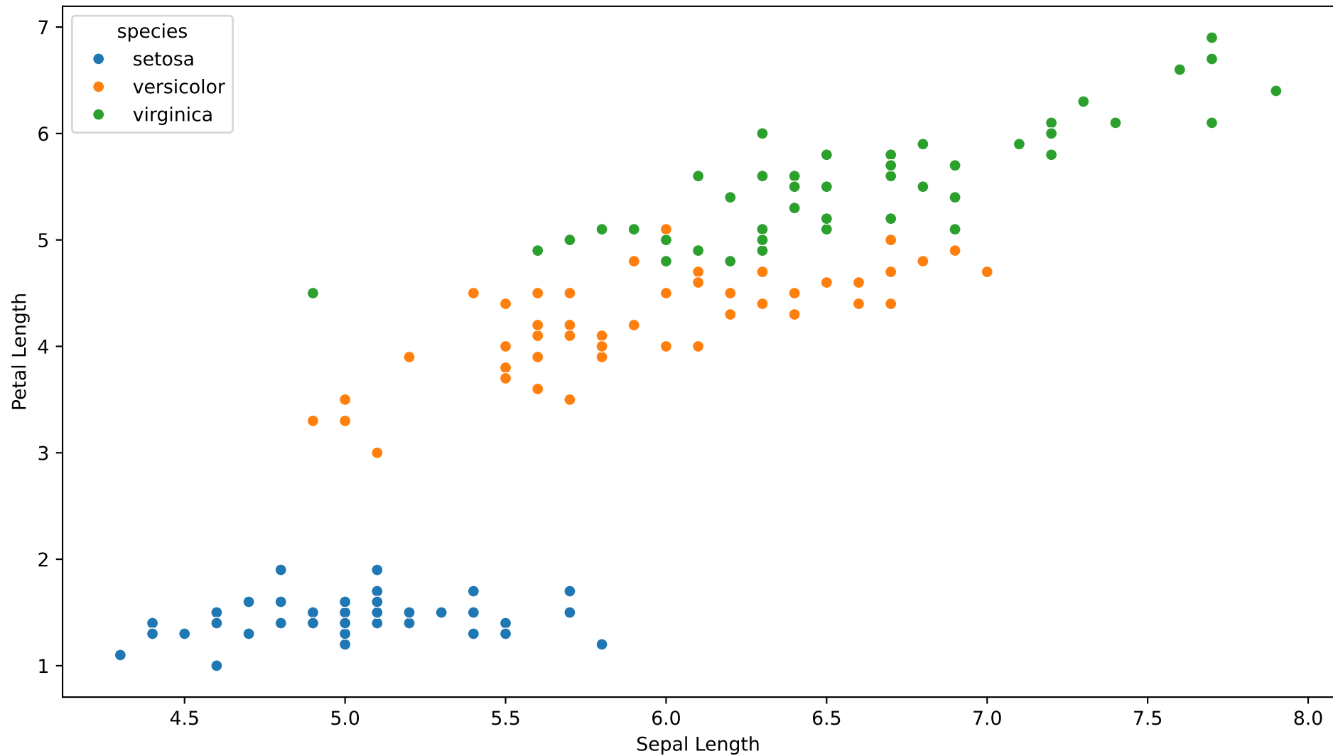
Figure 3: Sepal Length vs Petal Length
