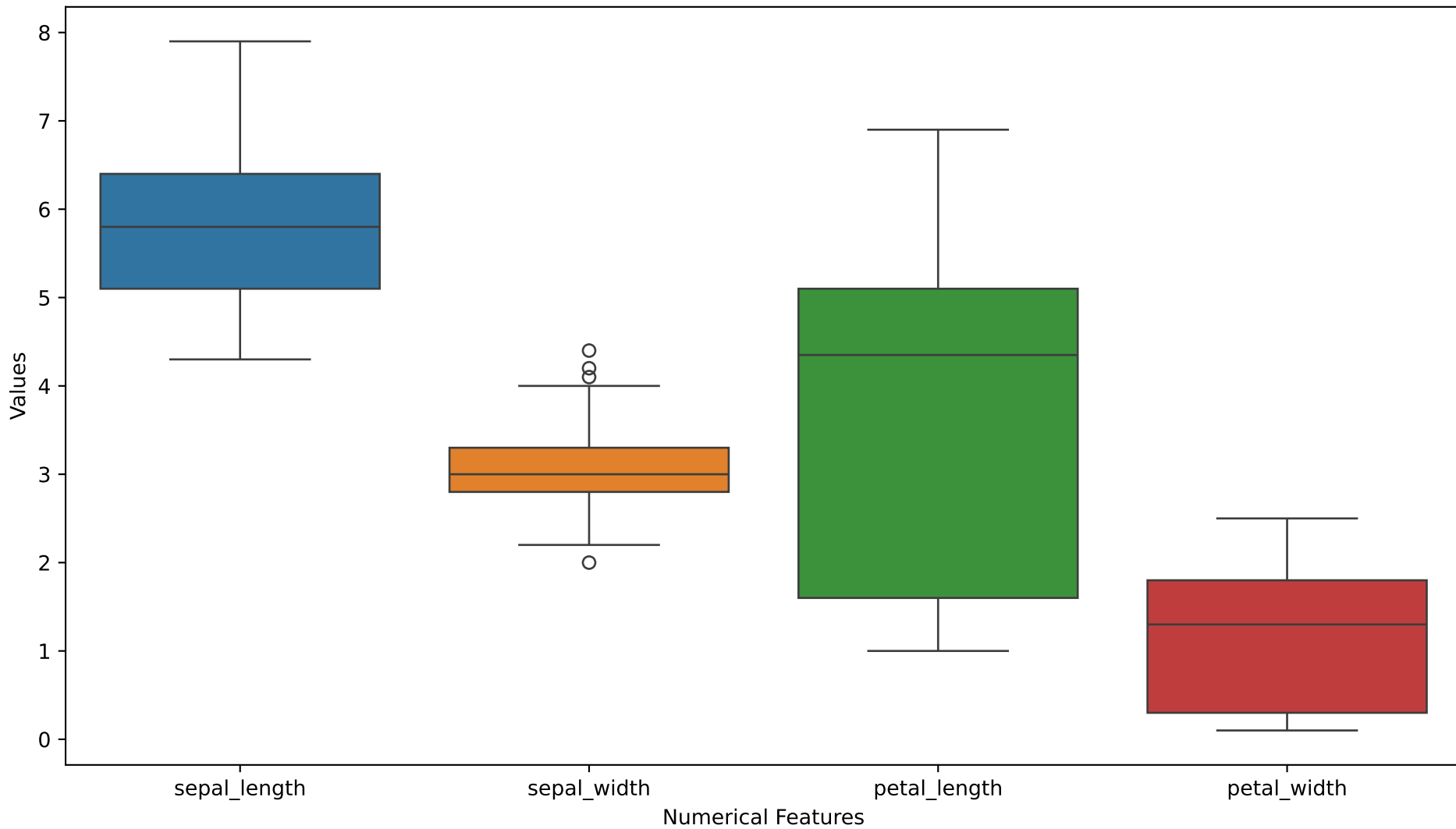
Figure 2: Boxplot of Numerical Features
