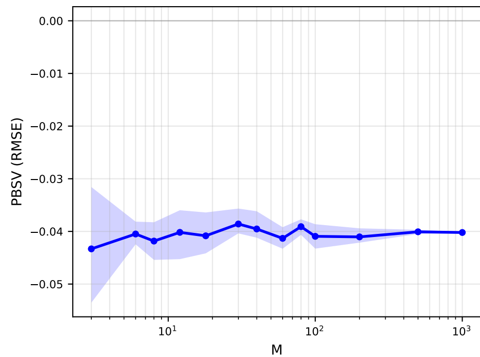
Fifth Predictor
