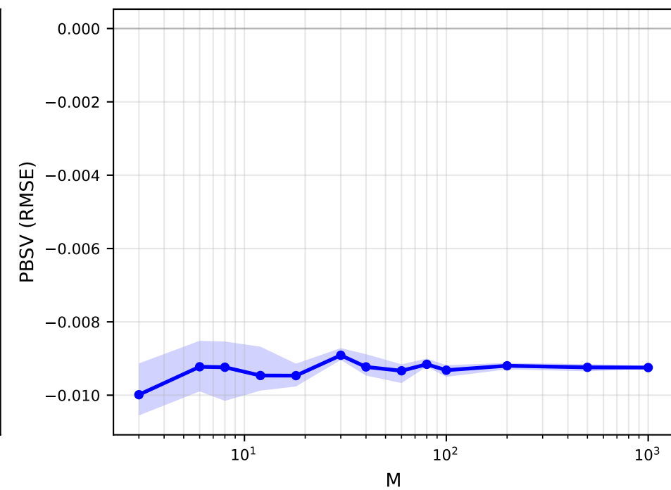
Sixth Predictor
