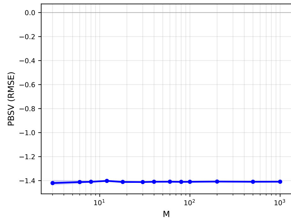
Fifth Predictor
