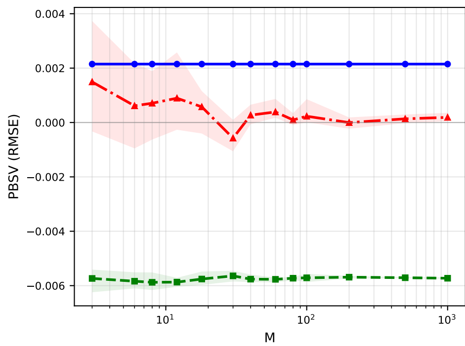
Sixth Predictor
