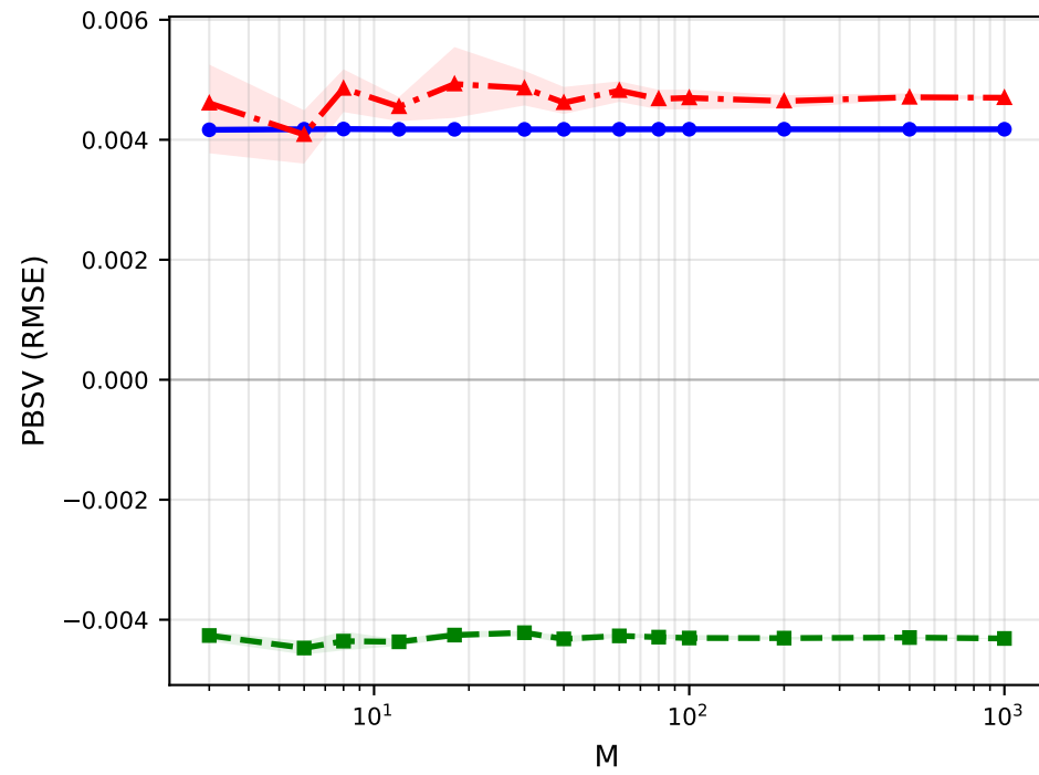
Fourth Predictor
