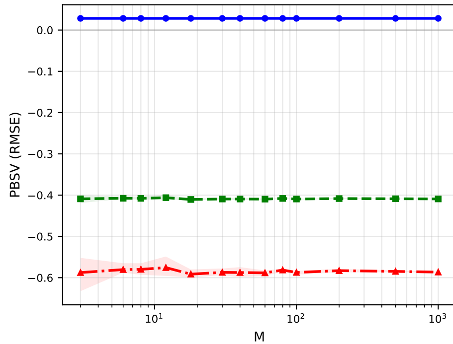
Fifth Predictor
