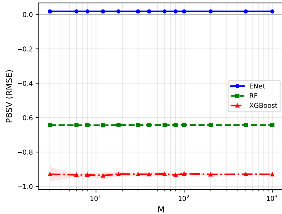
Fourth Predictor
