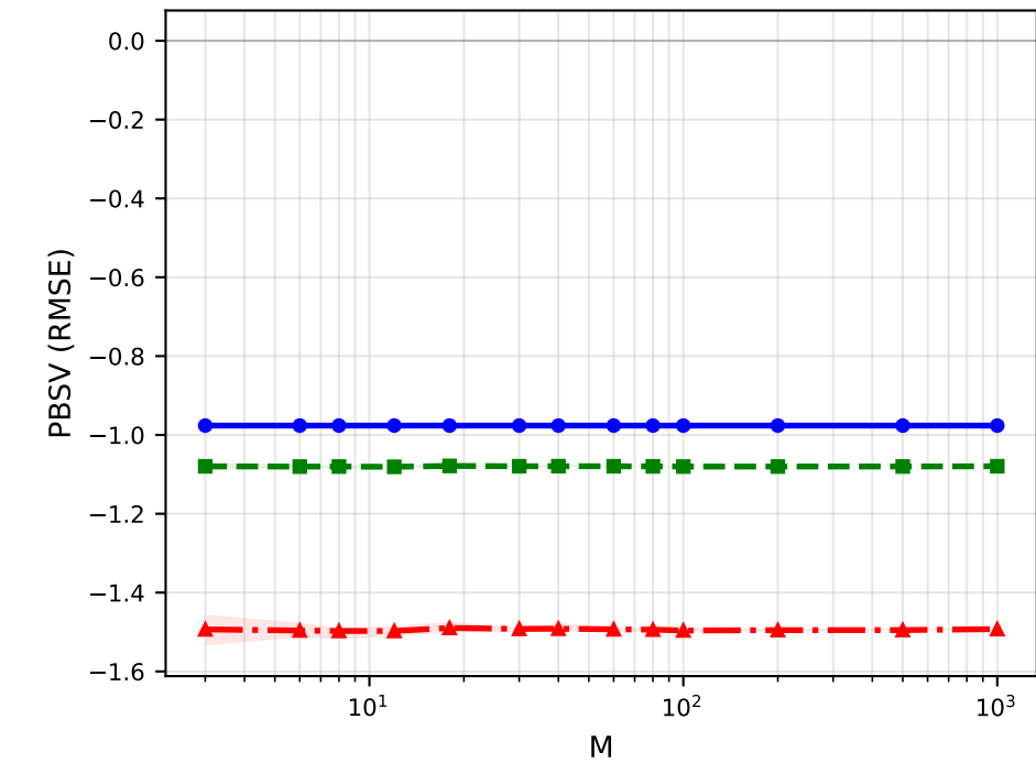
Sixth Predictor
