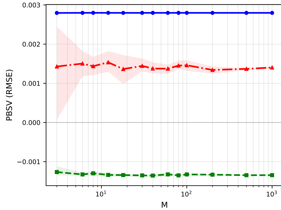
Fifth Predictor
