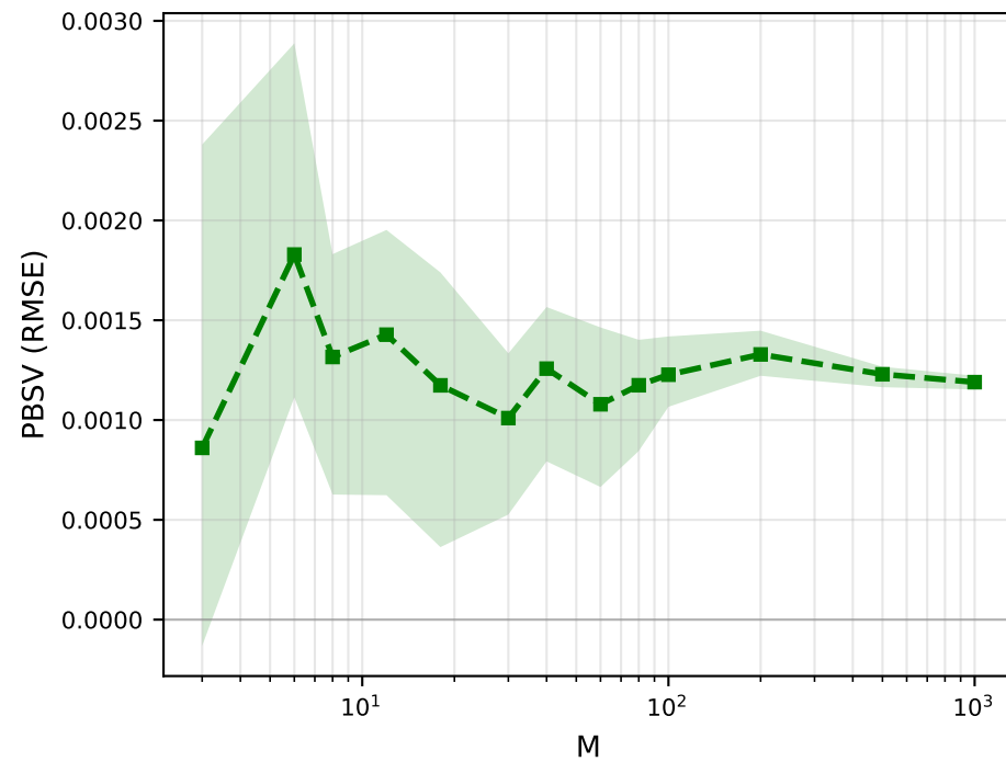
Fourth Predictor
