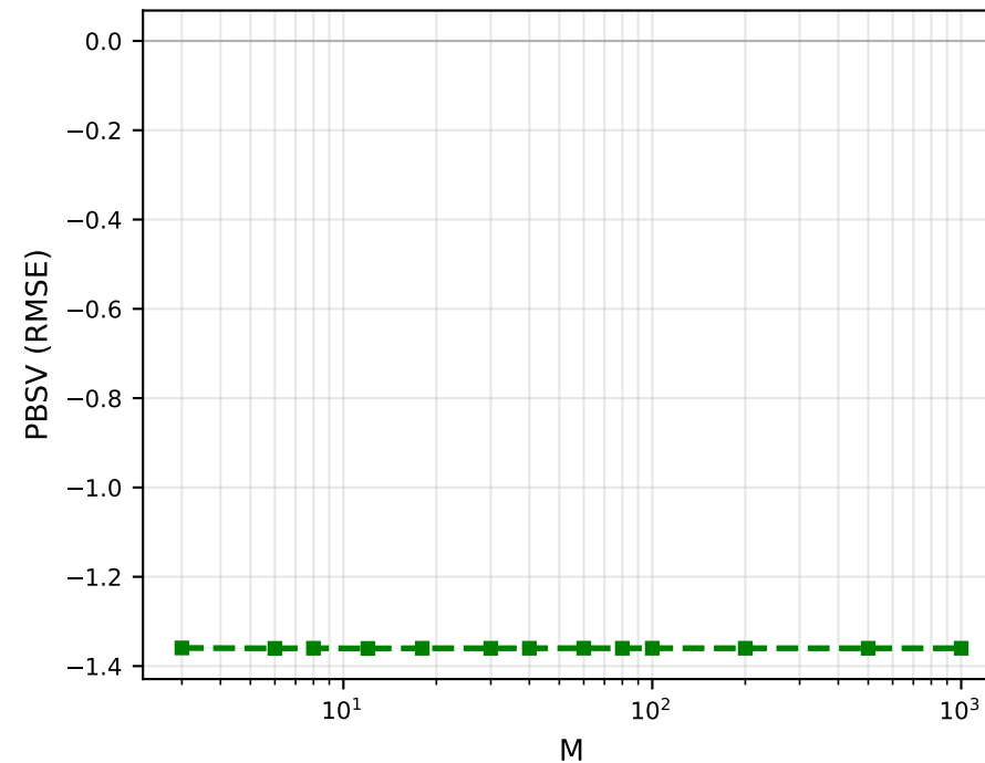
Fifth Predictor
