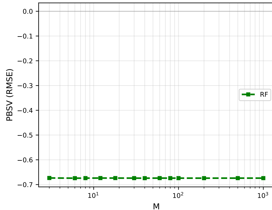
Fourth Predictor
