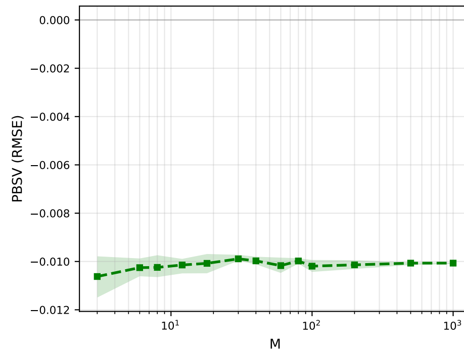
Fifth Predictor
