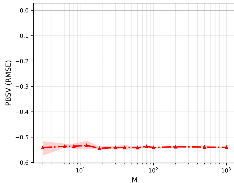
Fifth Predictor
