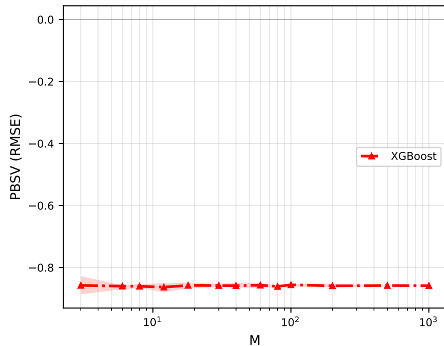
Fourth Predictor
