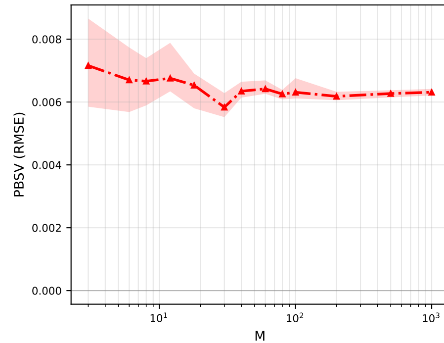
Sixth Predictor
