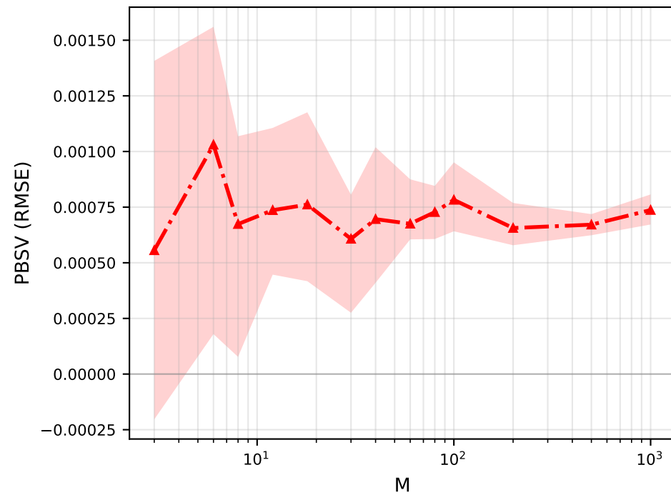
Fifth Predictor
