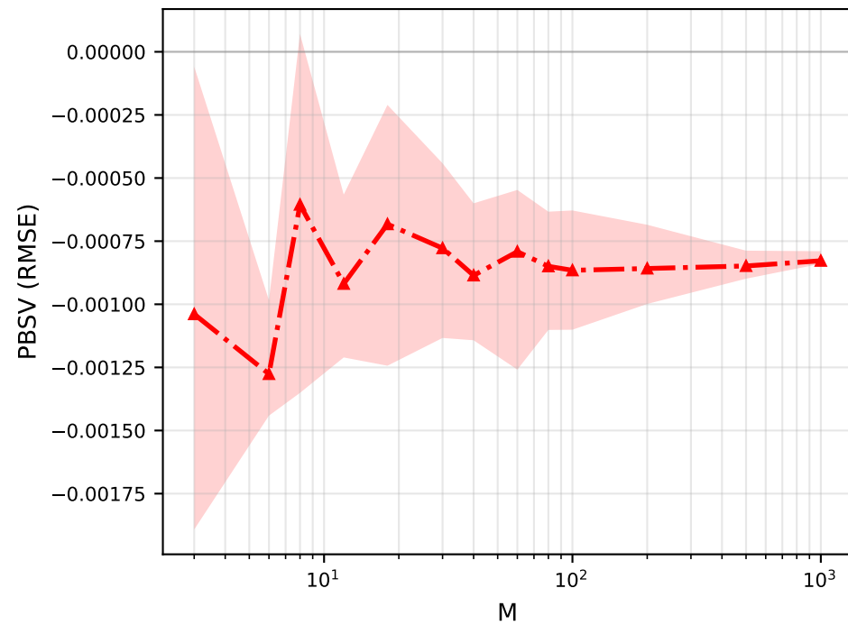
Fourth Predictor
