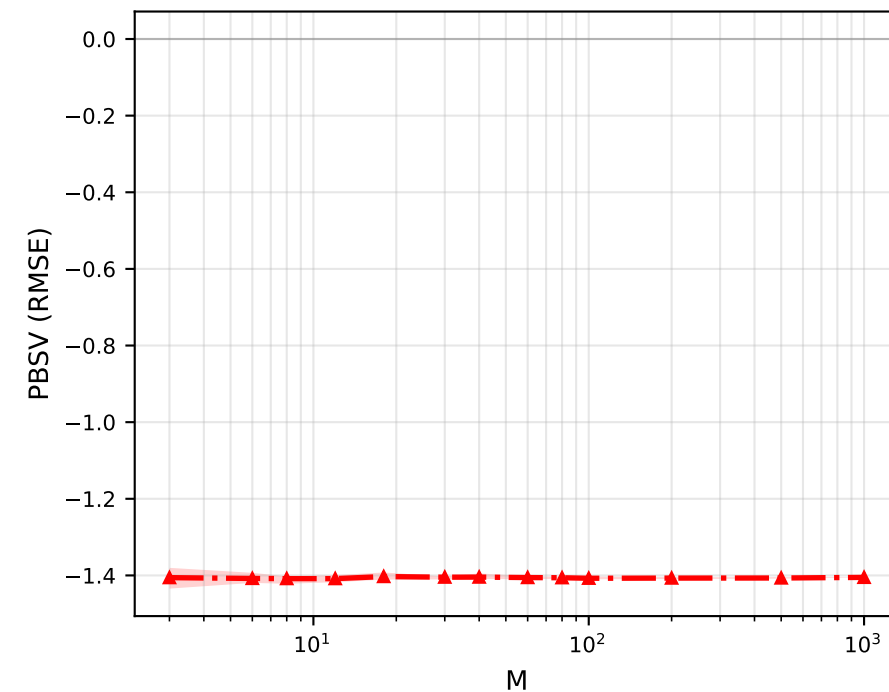
Sixth Predictor
