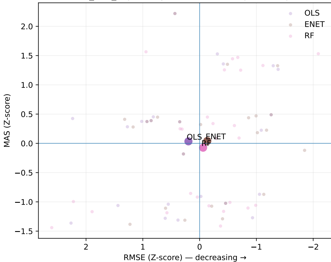
break_b15_expanding: MAS vs RMSE (quadrant plot)
