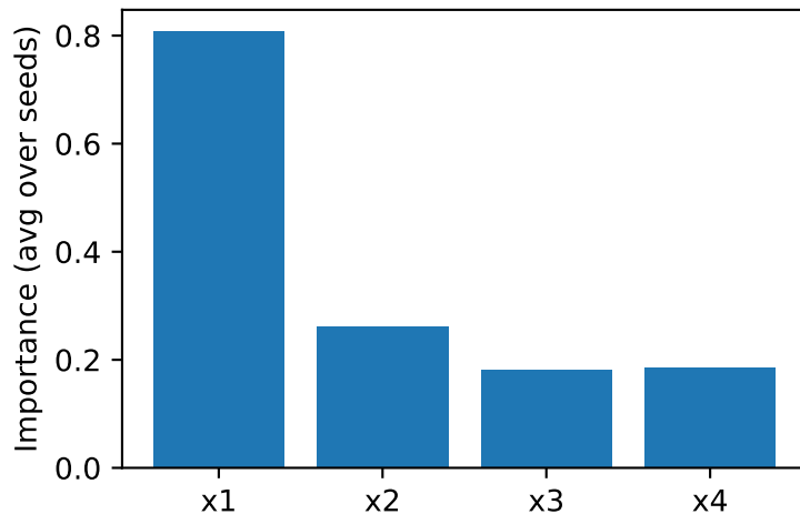
OLS: TS-Shapley-VI
