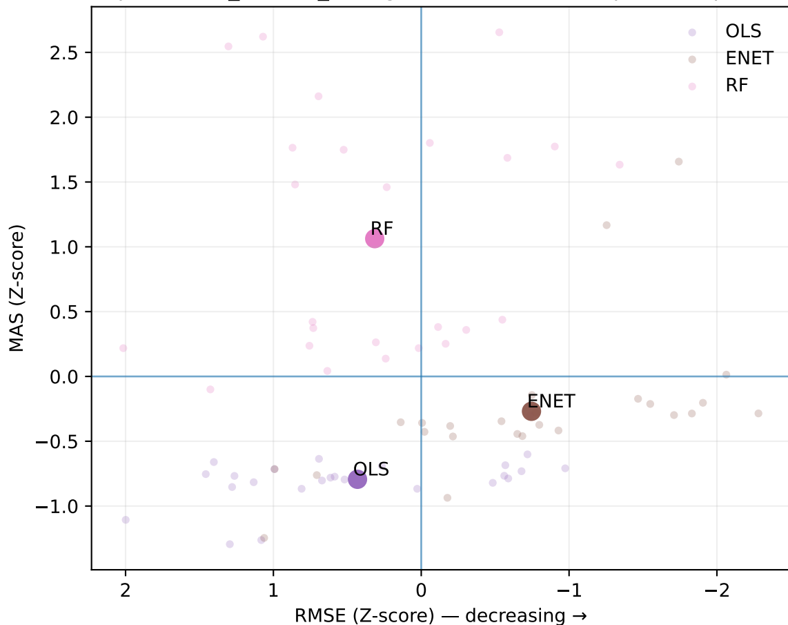
persistent_rho099_rolling20: MAS vs RMSE (quadrant plot)
