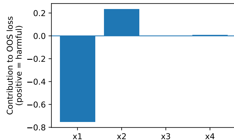
RF: GPBSV (MSE)
