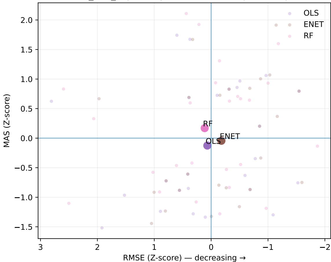
break_b08_expanding: MAS vs RMSE (quadrant plot)
