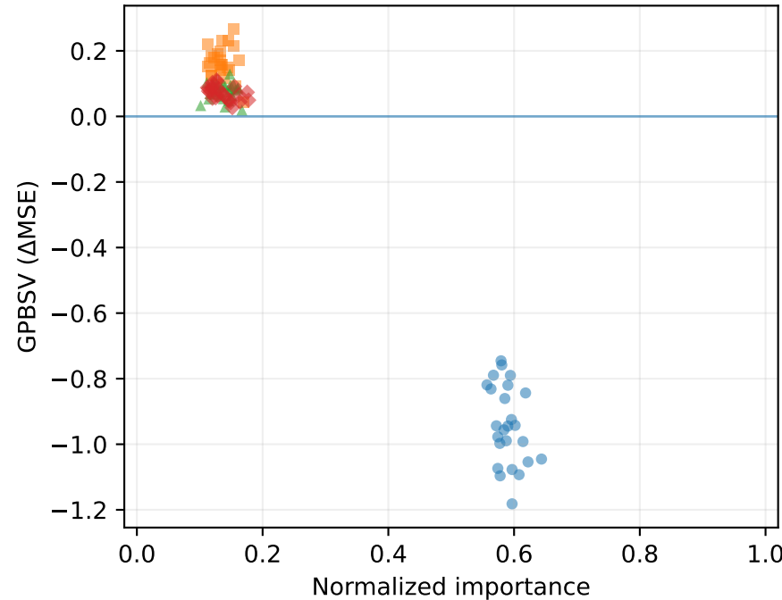
|t|-stat
