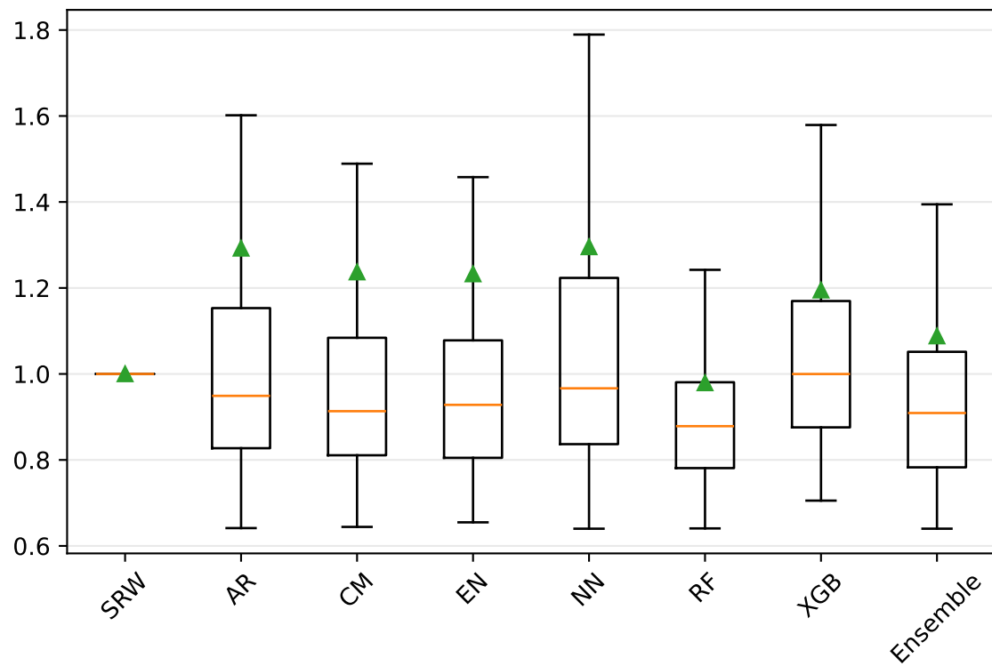
Forecast horizon: h = 12
