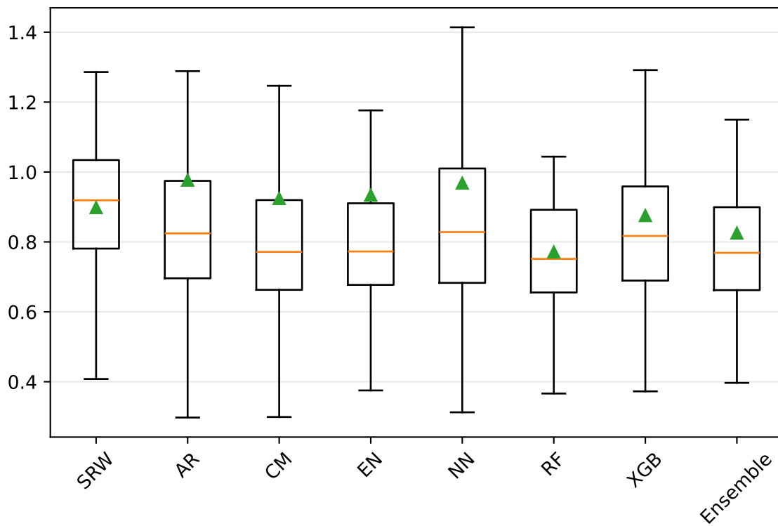
Forecast horizon: h = 6
