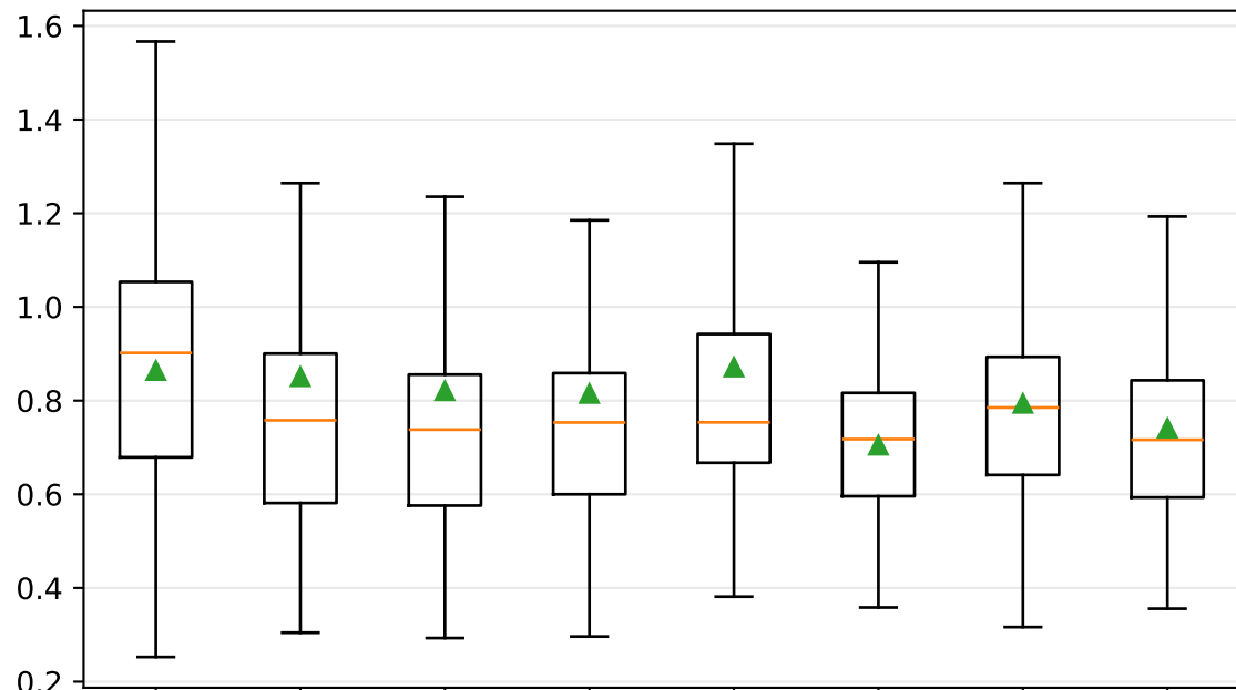
Forecast horizon: h = 3
