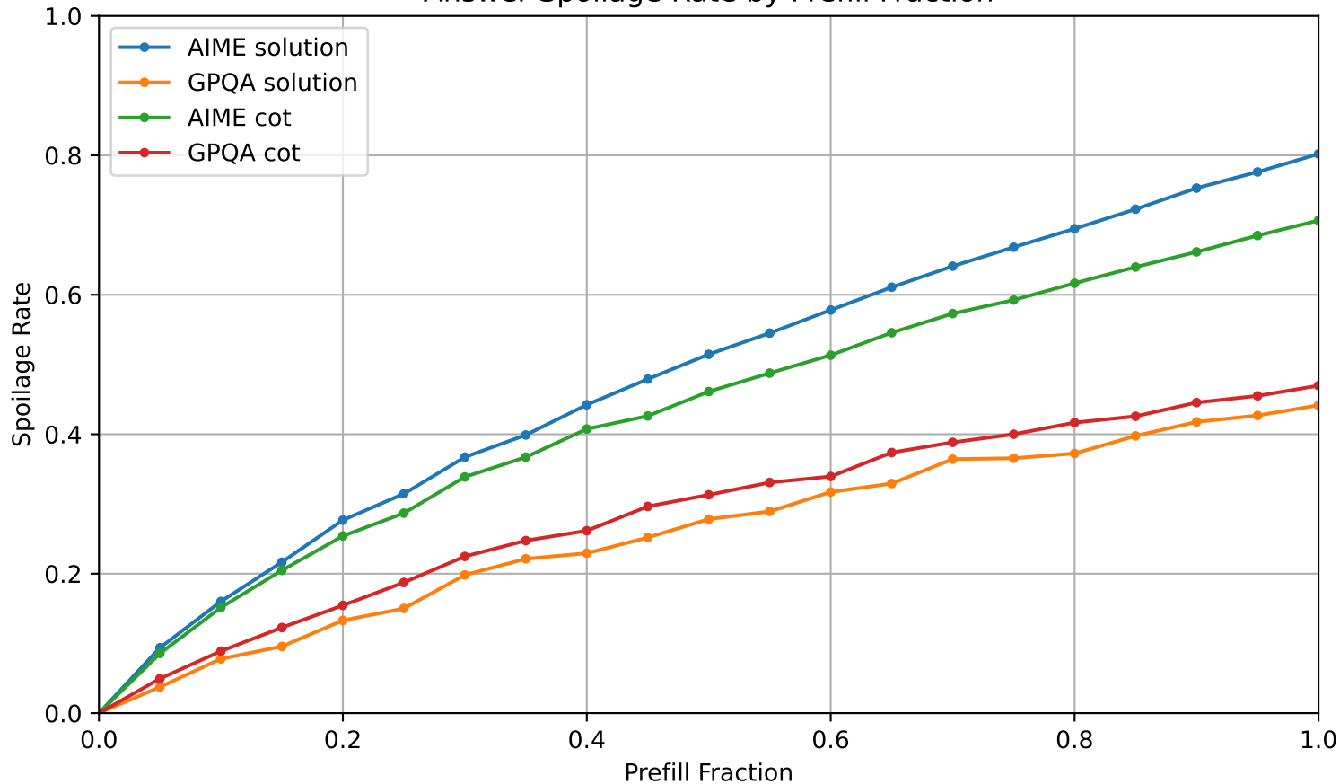
Answer Spoilage Rate by Prefill Fraction
