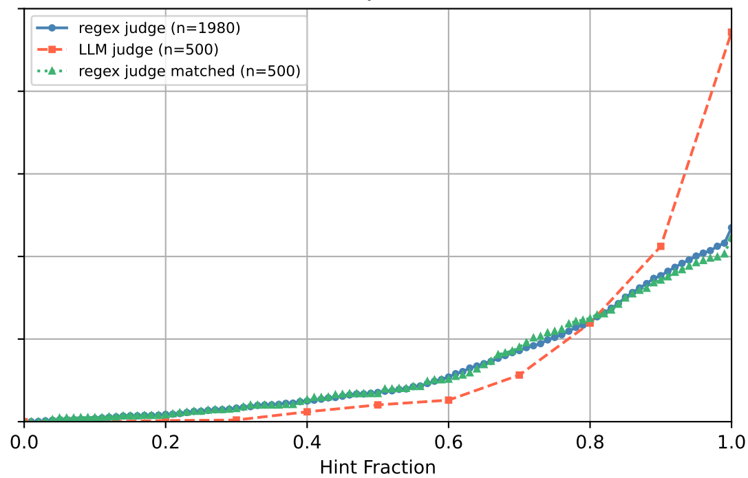
GPQA cot
