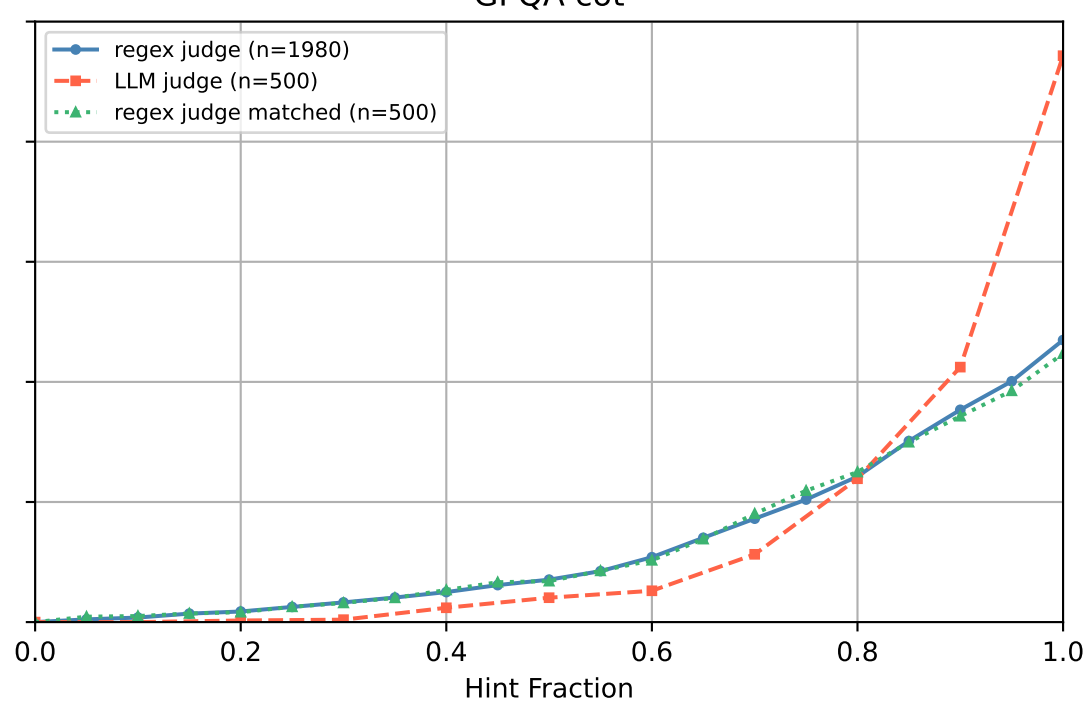
GPQA cot
