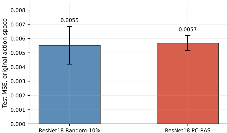
ResNet18 feature robustness
