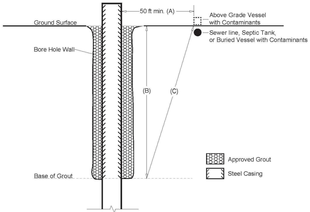
Figure 4b Minimum Distance from a Vessel Containing Contaminants
