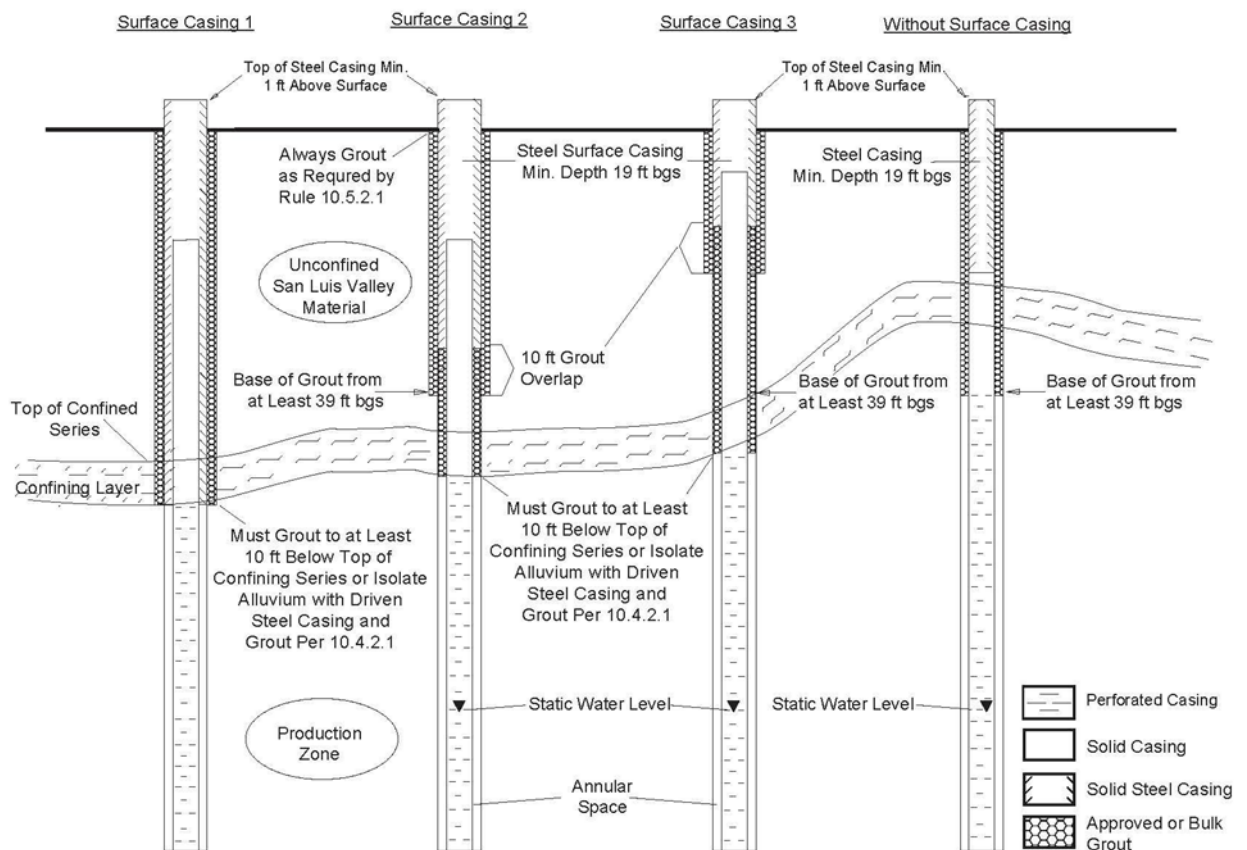
Figure 10. Schematic diagram for wells constructed into the Confined San Luis Valley aquifer
