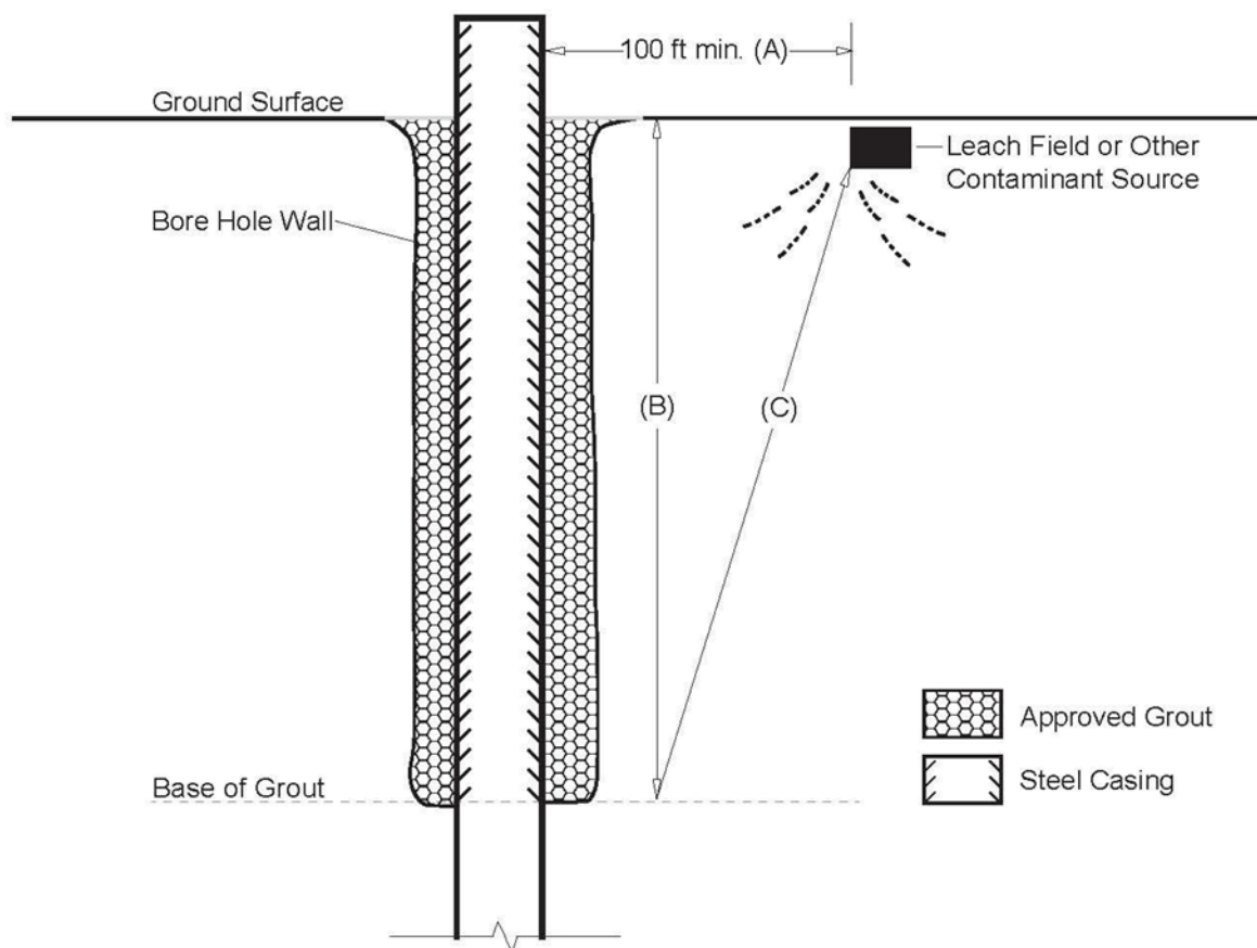
Figure 4a Minimum Distance from a Source of Contamination
