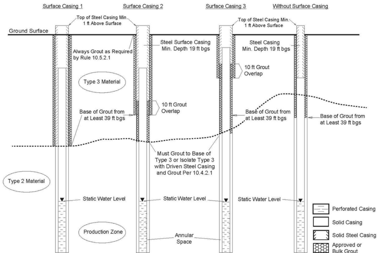
Figure 7b. Schematic diagram for wells constructed into Type 2 (unconfined bedrock) aquifers, overlain by a Type 3 (unconsolidated) aquifer.
