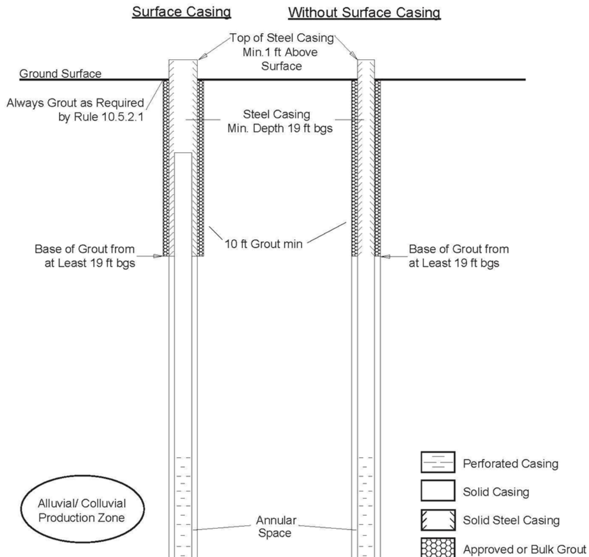
Figure 8. Schematic diagram for wells constructed into Type 3 (unconsolidated) aquifers.
