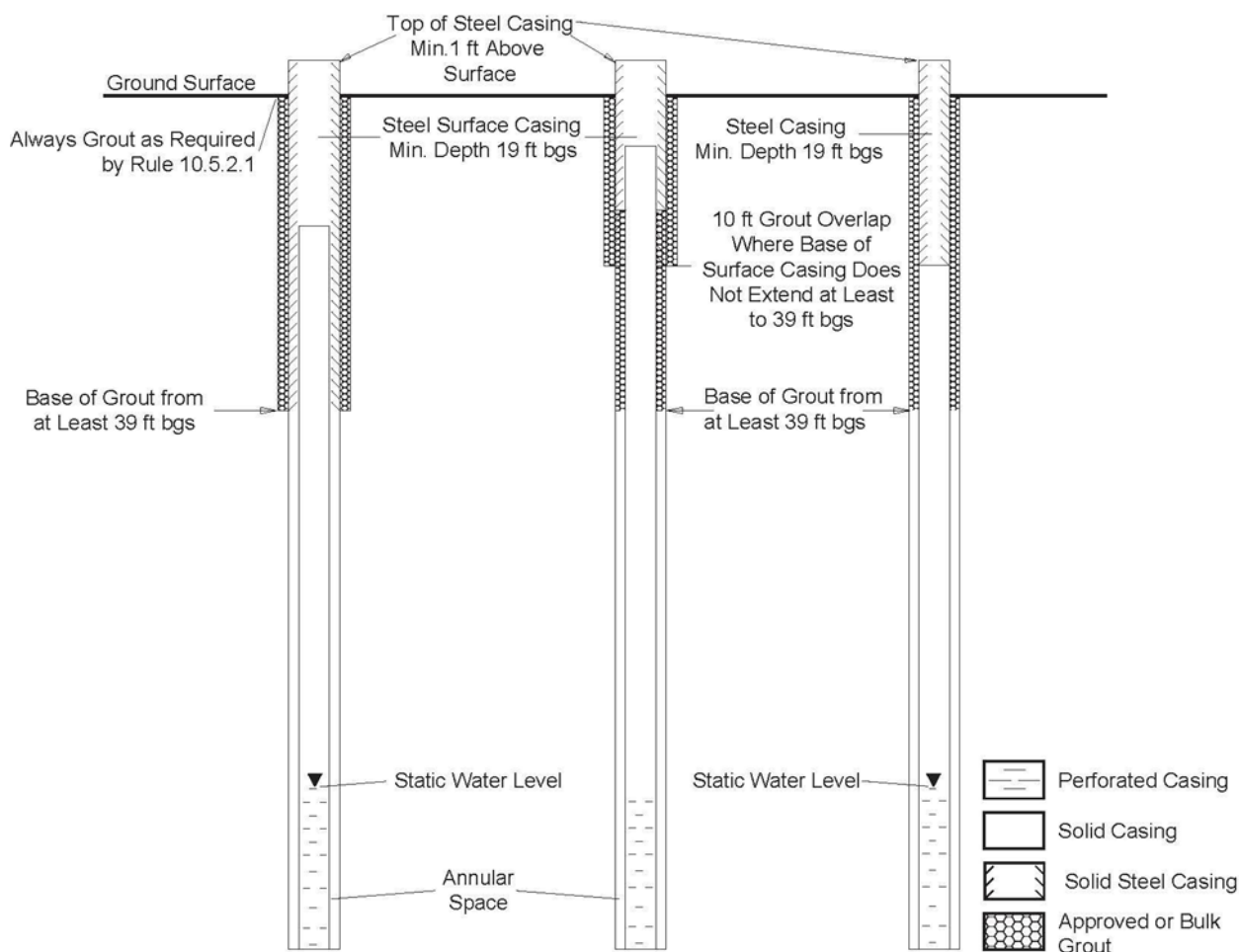
Figure 7a. Schematic diagram for wells constructed into Type 2 (unconfined bedrock) aquifers, not overlain by a Type 3 (unconsolidated) aquifer.
