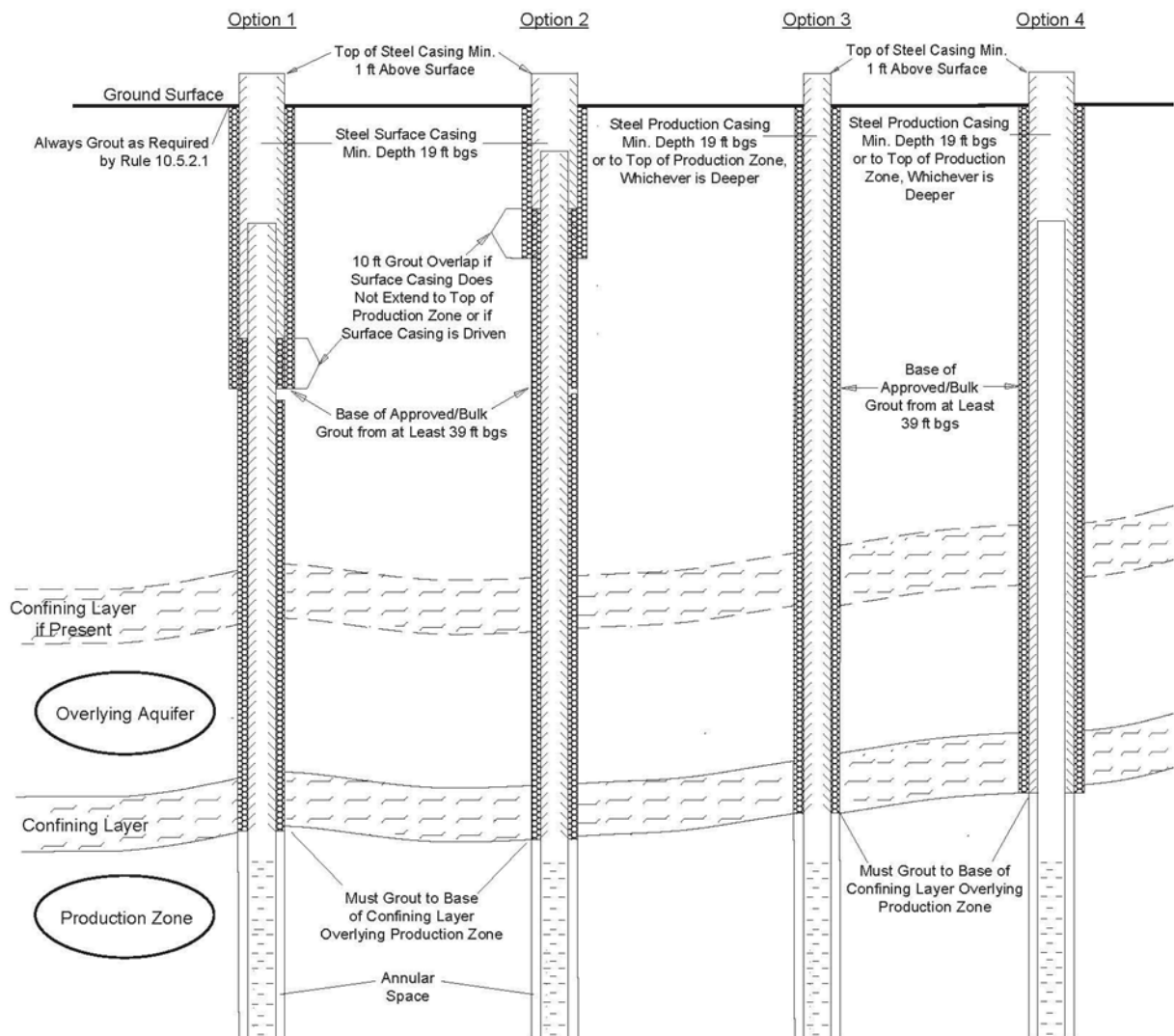
Figure 9. Schematic diagram for wells constructed into Laramie-Fox Hills aquifers inside and outside the Denver Basin.
