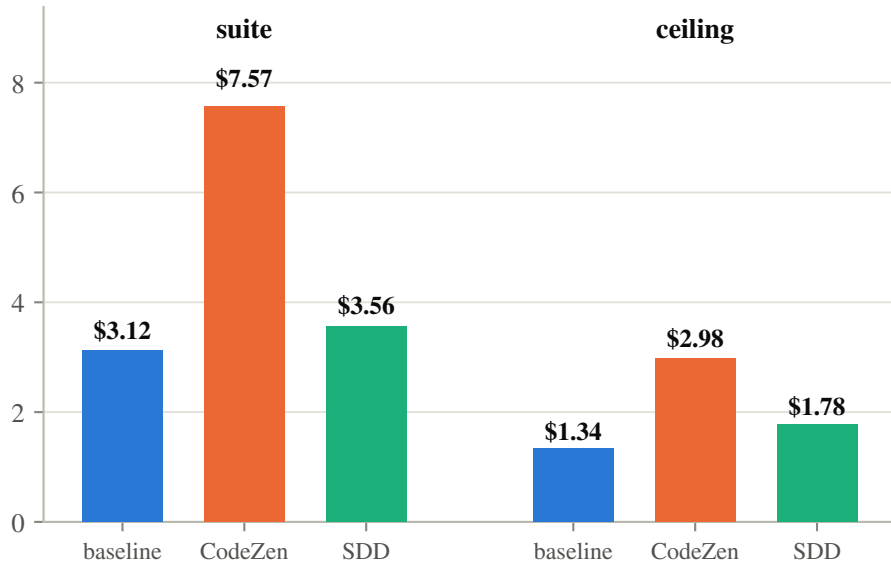
Spend per graded pass
