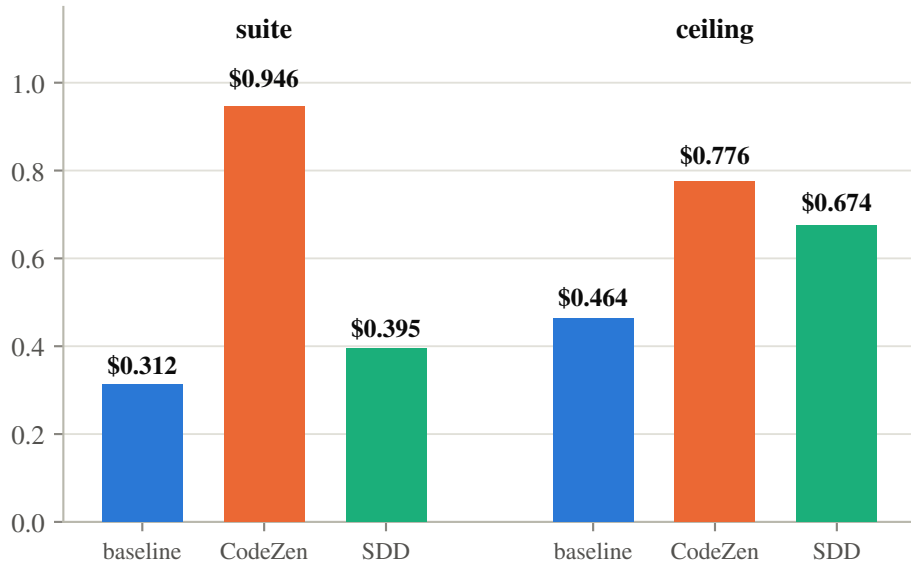
Spend per passing verifier test
