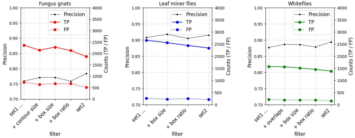
Figure 14: Results of different filters for each species. Results of the filters for each species. Left: parameter set 1 (no extra filtering). Right: parameter set 2 (all filters applied). Middle: individual filters added to set 1.
