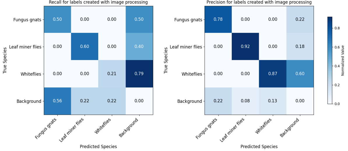
Figure 15: Confidence matrices for the image processed masks. Low recall is mainly due to the insects on the background structures that were masked out, which is why recall for the model trained on these labels increased (cf. Fig 11).
