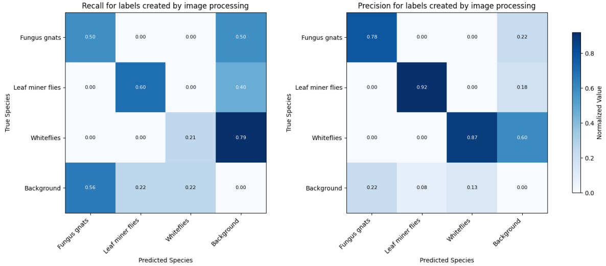
Figure 15: Confidence matrices for the image processed masks. Low recall is mainly due to the insects on the background structures that were masked out.
