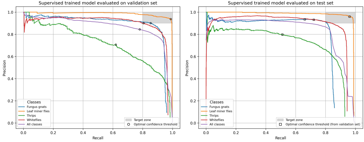
Figure 8: Precision-recall curves for the best model trained supervised on full images (S4). The left curve is taken on the validation set with the points closest to the target zone marked. The confidence thresholds associated with these points are used to predict on the test set. The right curve is taken on the test set with the arrived precision/recall values on the confidence thresholds. Training the model on the incomplete labels would still provide a sufficient model for all but the thrips, however deriving the confidence thresholds from the incomplete labels makes the model miss its best performance on the completely labeled test set.
