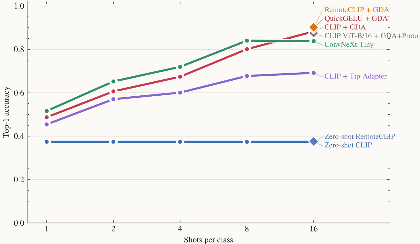
Eurosat: Accuracy vs. Support Size
