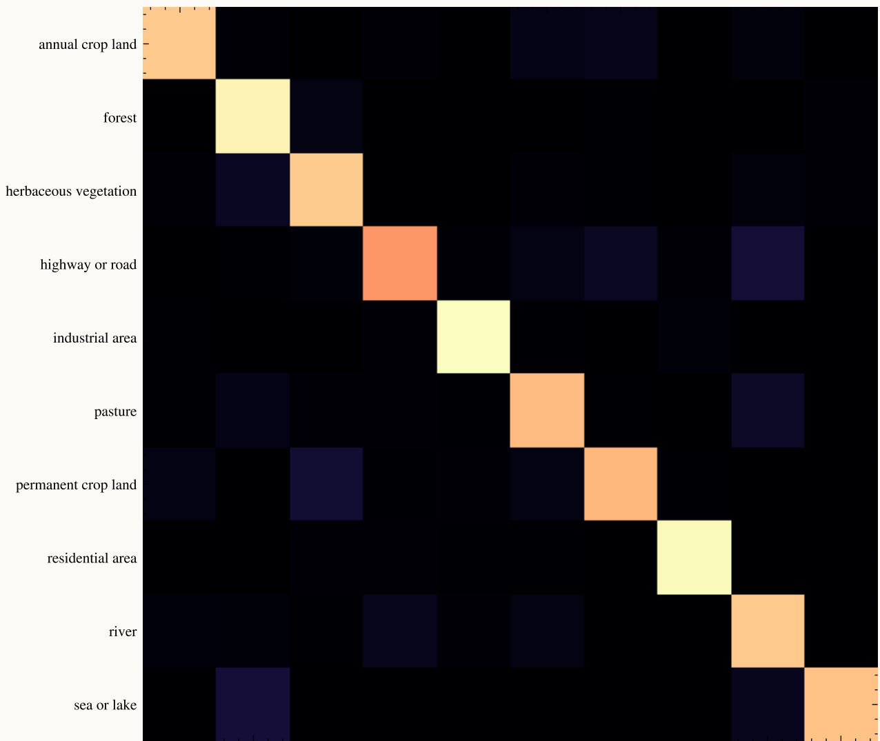
Normalized Confusion Matrix: CLIP ViT-B/16 + GDA+Proto
