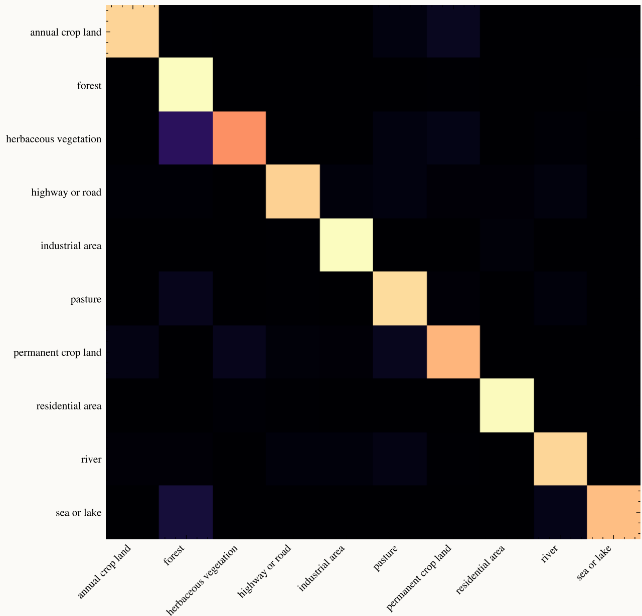
Normalized Confusion Matrix: CLIP ViT-B/16-QuickGELU + GDA
