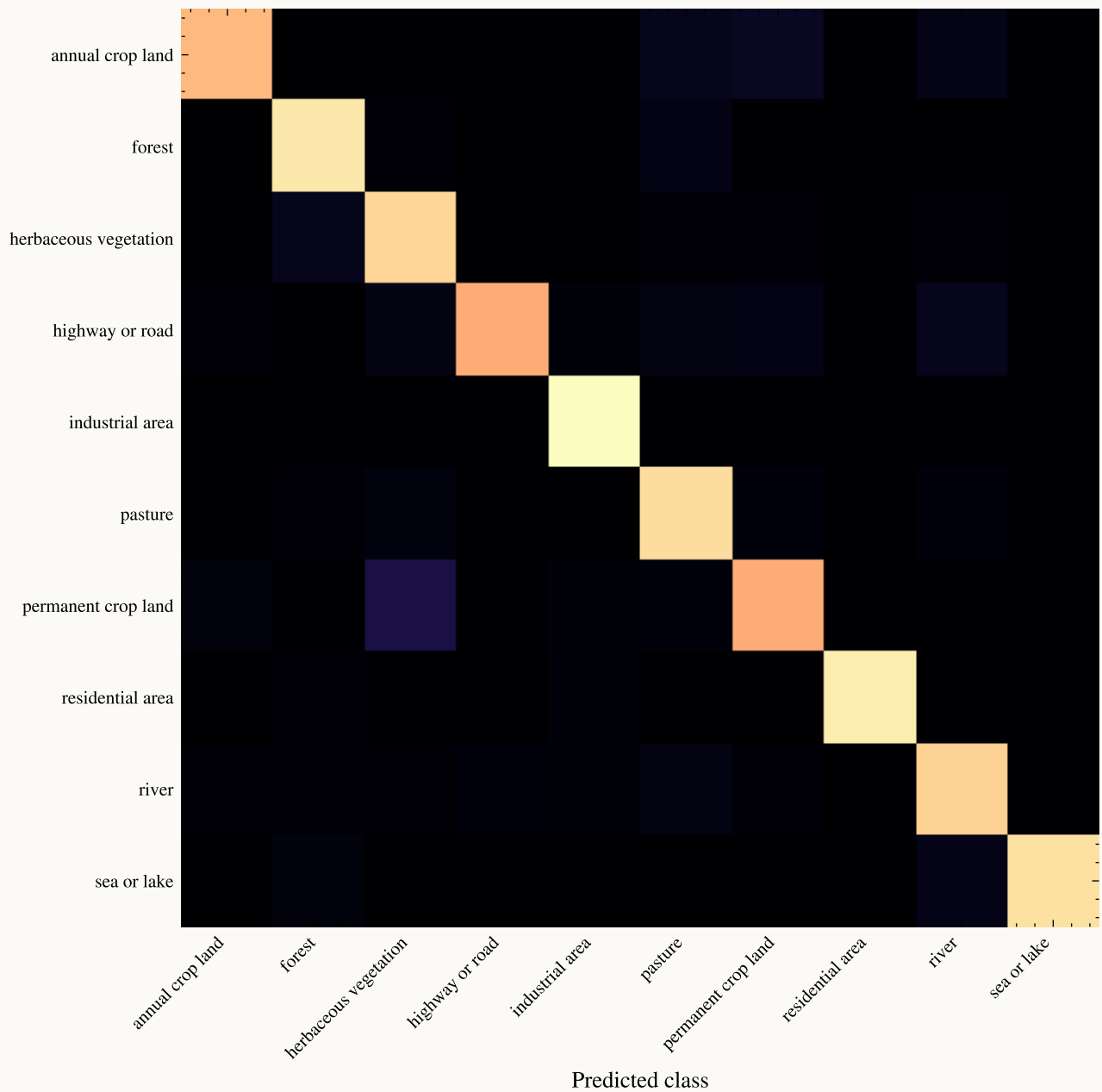
Normalized Confusion Matrix: RemoteCLIP ViT-B/32 + GDA
