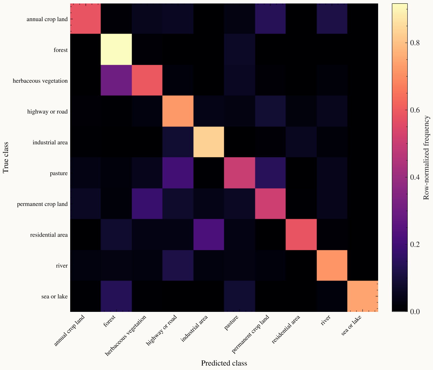
Normalized Confusion Matrix: CLIP ViT-B/16 + GDA
