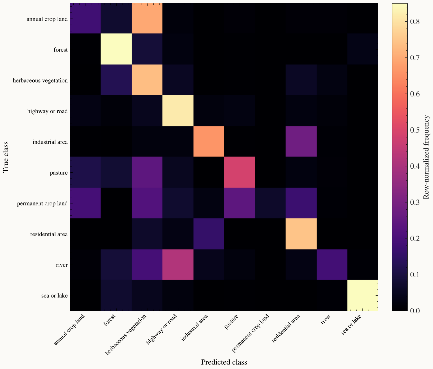
Normalized Confusion Matrix: CLIP ViT-B/16 + Tip-Adapter
