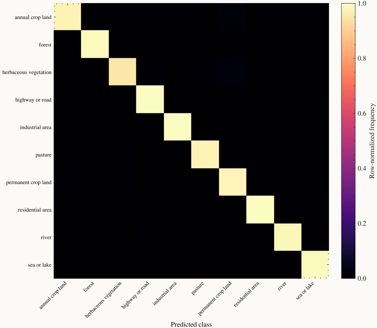
Normalized Confusion Matrix: ConvNeXt-Tiny Full Fine-Tune
