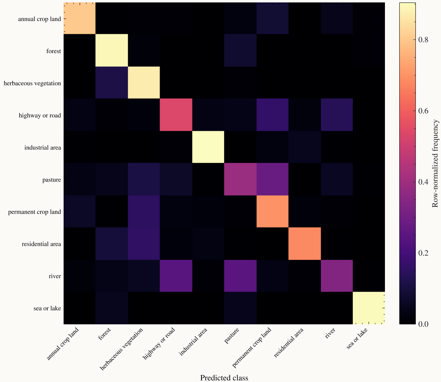
Normalized Confusion Matrix: ConvNeXt-Tiny
