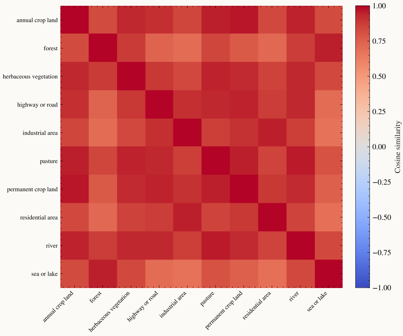
Class Centroid Cosine Similarity
