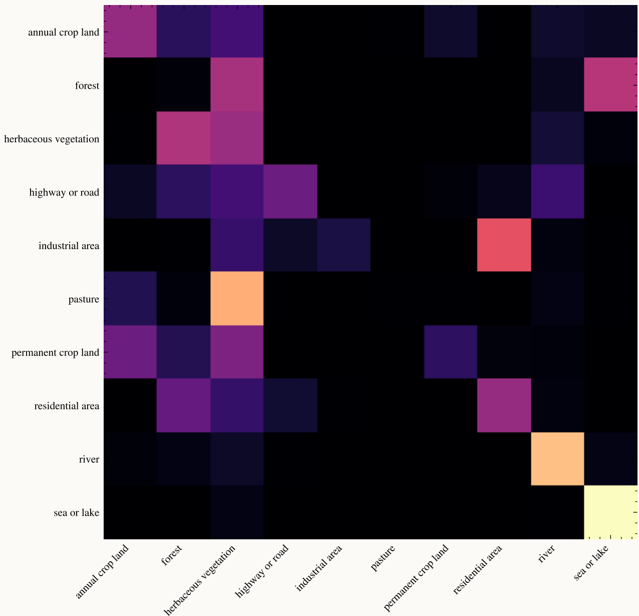
Normalized Confusion Matrix: Zero-shot RemoteCLIP ViT-B/32
