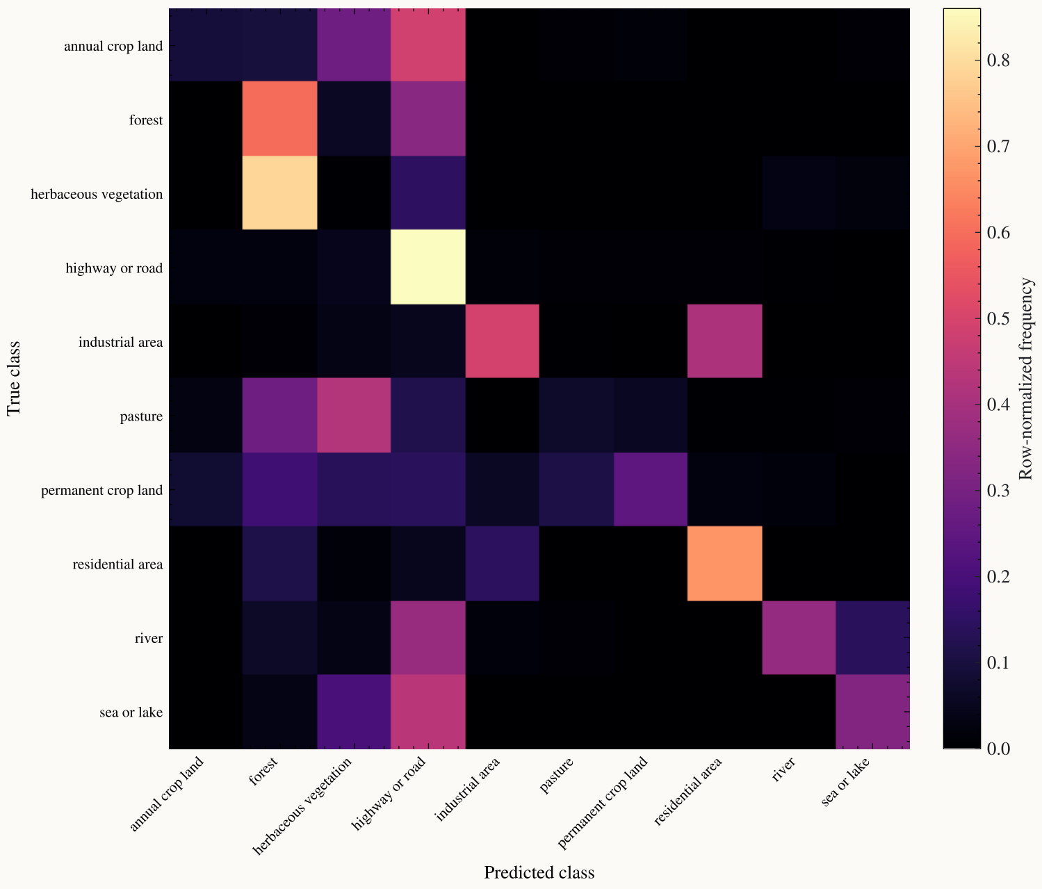
Normalized Confusion Matrix: Zero-shot CLIP ViT-B/16
