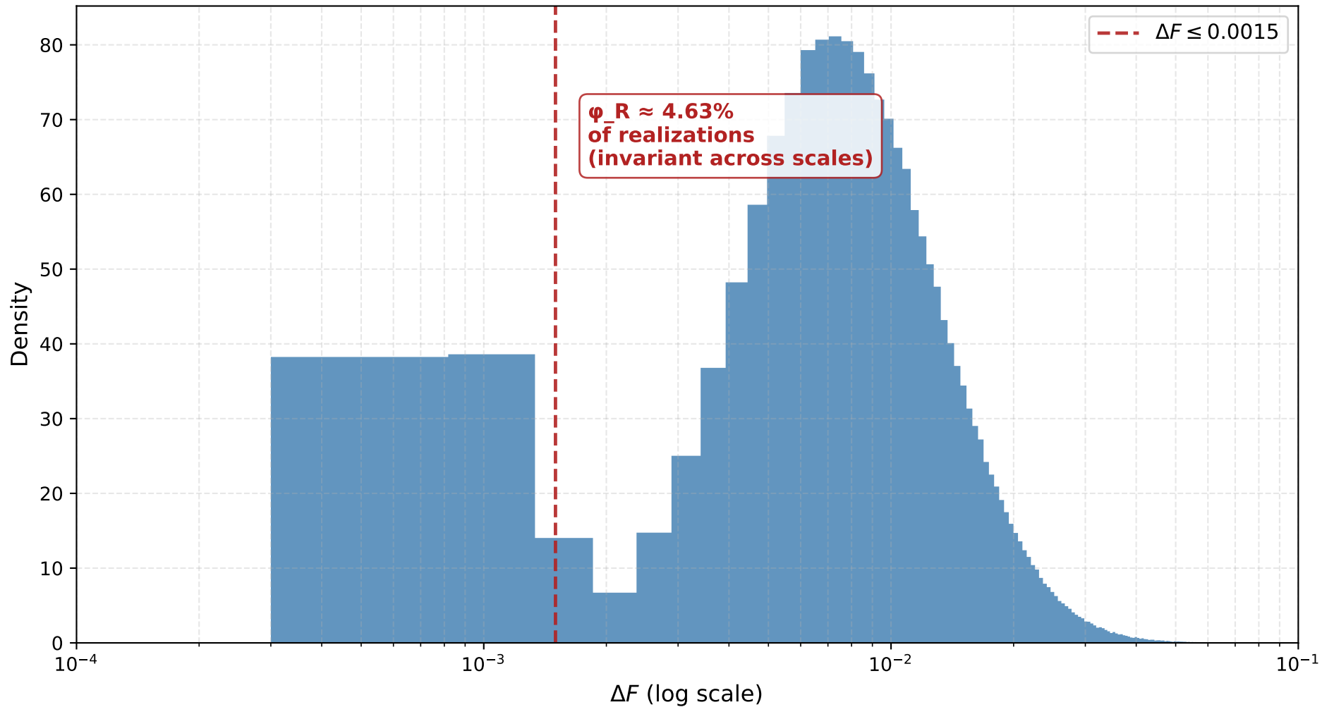
Distribution of Surprise Minimization ( \Delta F ) in Large Collectives (example from n \approx 10^7 dyads)
