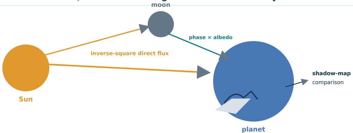
Figure 9: The Sun contributes direct flux to each body, the Moon reflects a phase-dependent portion toward the planet, and terrain visibility controls direct light. The diagram is schematic; arrow widths do not encode flux.
