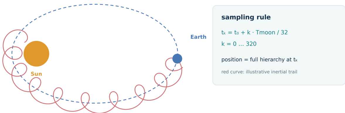
Figure 8: Illustrative moon trail in the inertial world frame. The repeated local cycles travel with the parent; the curve is explanatory and does not plot a measured scenario trajectory. Generated schematic.
