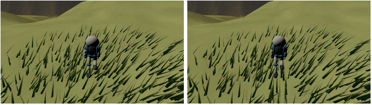
Figure 27: Identical pose, terrain, foliage roots and wind phase: unpressed control (left), persistent walking trail (right). The six-metre walk records 20 segments with 977 GPU-submitted blades; its replay is byte-identical.
