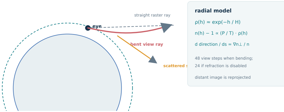
Figure 11: A refractive view ray bends through denser air while solar light contributes scattered radiance. Near terrain keeps its rasterized silhouette; only visible distant imagery is reprojected. Generated schematic.
