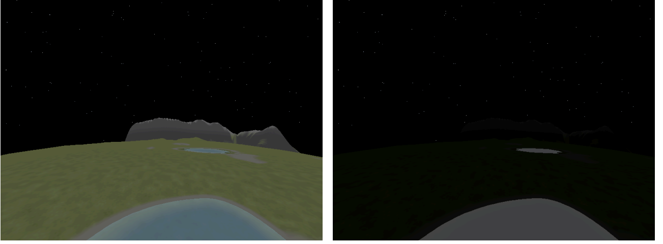
Figure 12: A controlled night-scene comparison from the current gallery: moonlit (left) and moonless (right). The saved replays preserve camera and lighting inputs, allowing the reflected-light term to be isolated.
