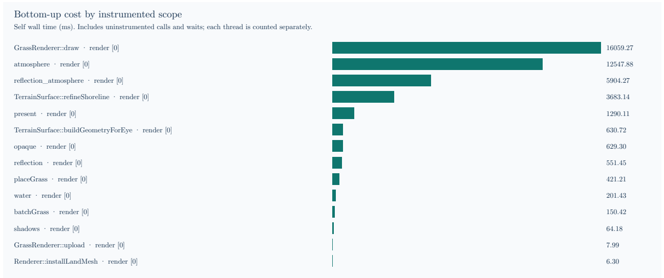
Figure 24: Bottom-up self wall time over ten walking frames. Immediate child scopes are subtracted; uninstrumented work and waits remain.
