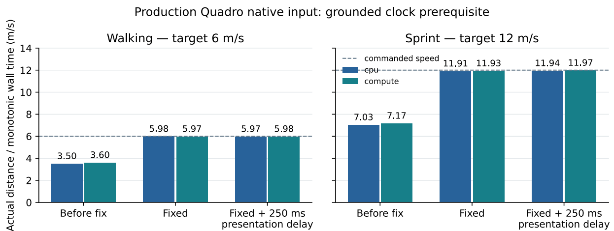
Figure 8: Actual grounded distance per monotonic wall second on production Quadro native input. Baseline uses short routes; fixed natural and delayed checks use 100 m. Each bar is one input run, with full raw spikes retained; these are speed prerequisites, not paired route cost acceptance or uncertainty estimates.
