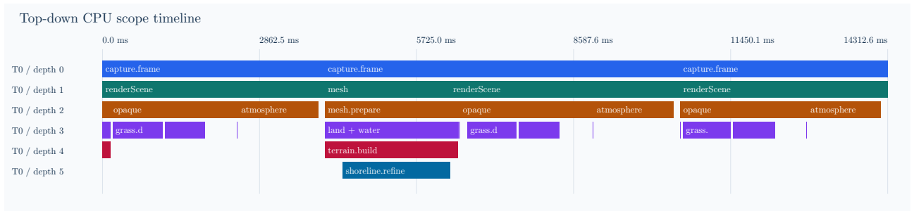
Figure 23: Top-down nested CPU scope timeline for three frozen walking frames on llvmpipe. Width represents wall time, including waits.
