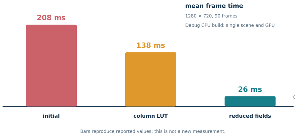
Figure 17: Reported mean frame times from README.md, Quadro M1000M, 1280 \times 720 , 90 frames. These bars visualize previously reported measurements, not a new benchmark.
