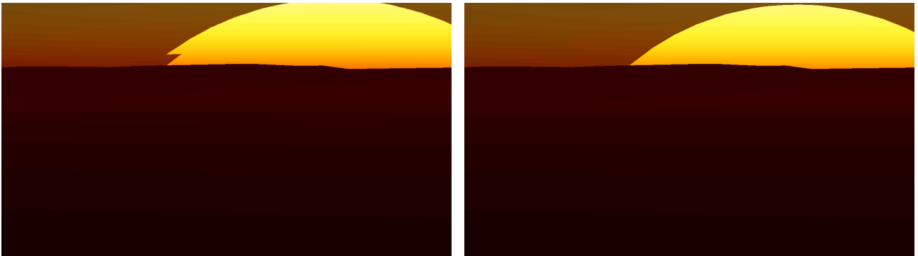
Figure 14: Matched full-resolution renderer captures of extreme refraction enabled (left) and disabled (right). Only the JSON bending switch changes; scattering and exposure remain active in both.
