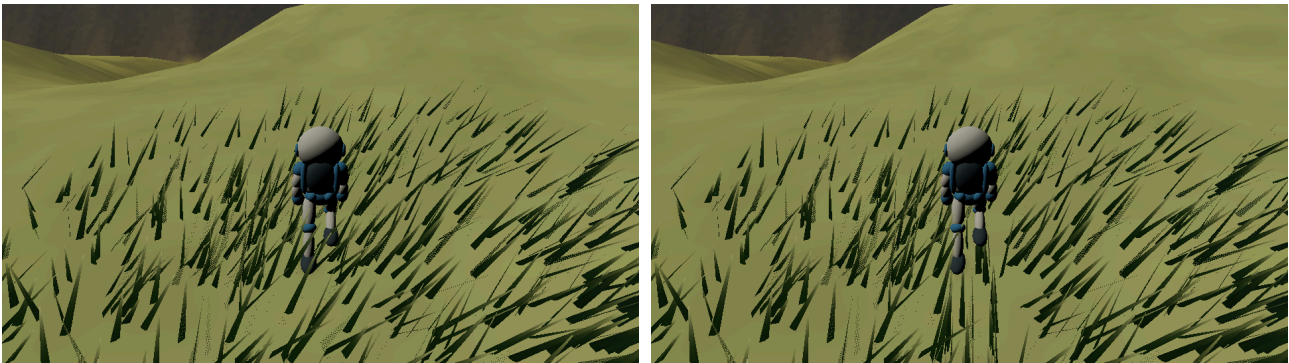
Figure 34: Identical pose, terrain, foliage roots and wind phase: unpressed control (left), persistent walking trail (right). The six-metre walk records 20 segments with 977 GPU-submitted blades; its replay is byte-identical.
