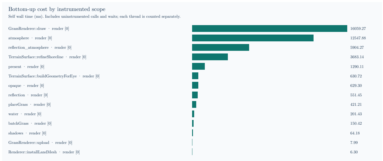
Figure 28: Bottom-up self wall time over ten walking frames. Immediate child scopes are subtracted; uninstrumented work and waits remain.
