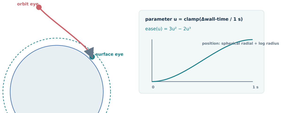
Figure 33: Orbit-to-surface descent. The curve shows the implemented smoothstep parameter; the spatial path is schematic because the actual start, target, and terrain vary by scene.
