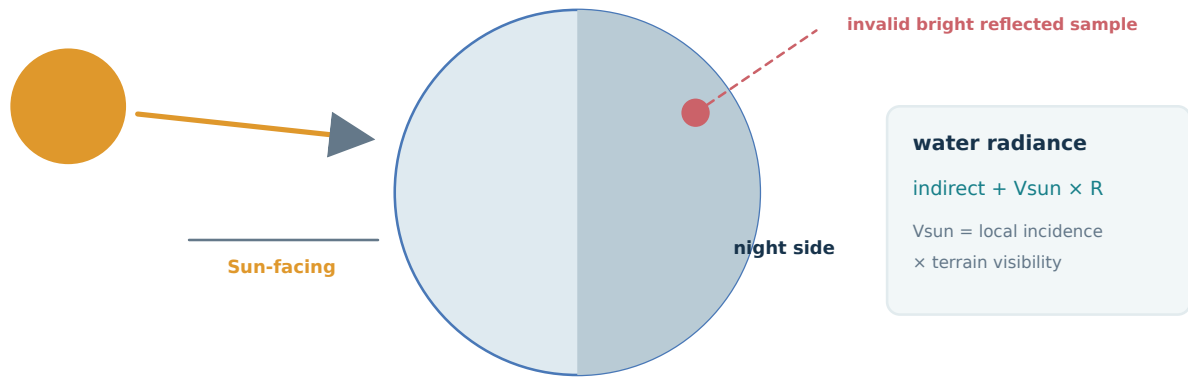
Figure 31: A reflected bright sample can exist in image space even when the water point lies on the night side. Local incidence and shadow-map visibility gate the direct reflection term. Generated schematic.
