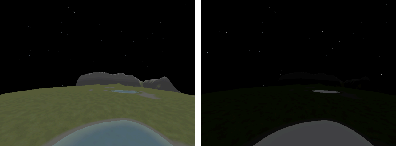
Figure 16: A controlled night-scene comparison from the current gallery: moonlit (left) and moonless (right). The saved replays preserve camera and lighting inputs, allowing the reflected-light term to be isolated.
