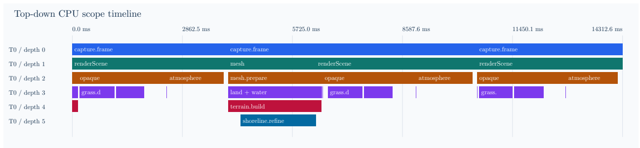
Figure 27: Top-down nested CPU scope timeline for three frozen walking frames on llvmpipe. Width represents wall time, including waits.
