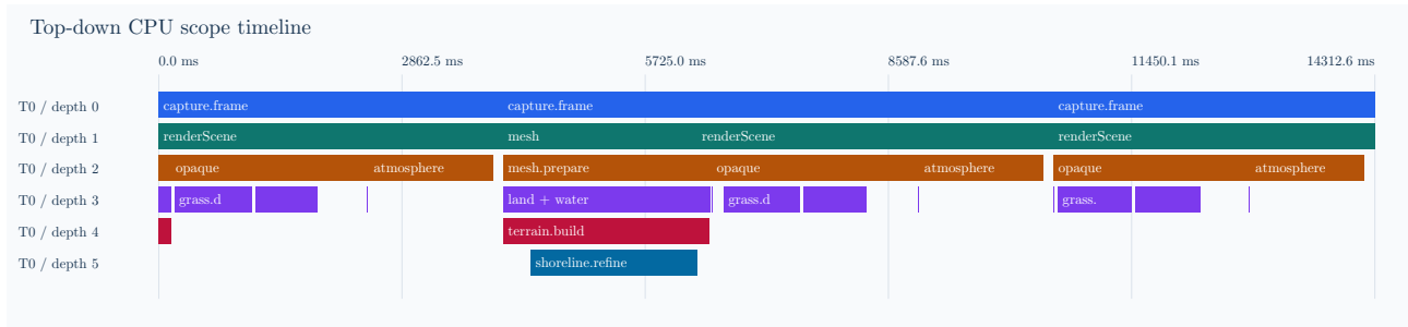
Figure 18: Top-down nested CPU scope timeline for three frozen walking frames on llvmpipe. Width represents wall time, including waits.
