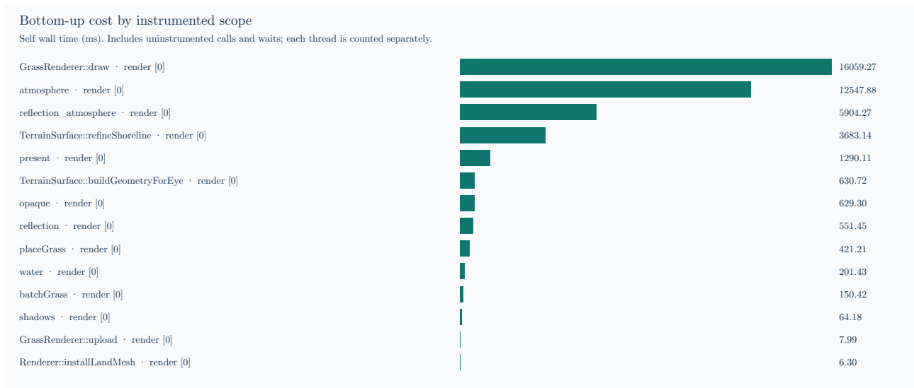
Figure 19: Bottom-up self wall time over ten walking frames. Immediate child scopes are subtracted; uninstrumented work and waits remain.
