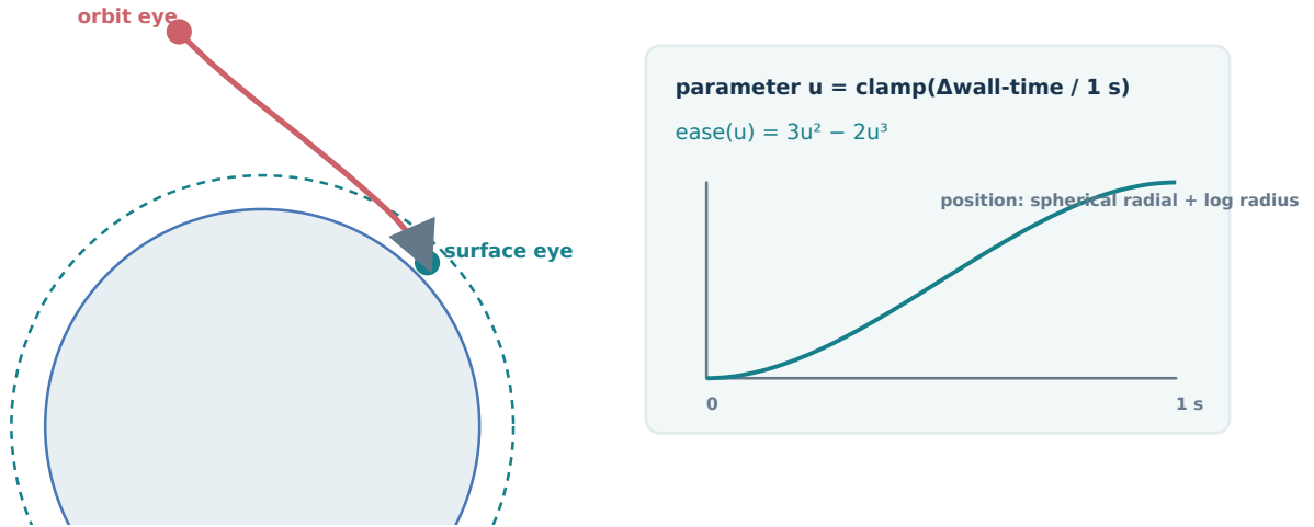
Figure 23: Orbit-to-surface descent. The curve shows the implemented smoothstep parameter; the spatial path is schematic because the actual start, target, and terrain vary by scene.
