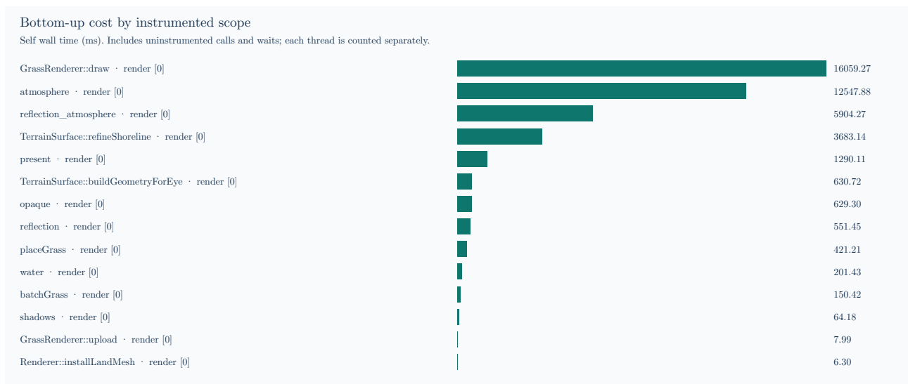
Figure 18: Bottom-up self wall time over ten walking frames. Immediate child scopes are subtracted; uninstrumented work and waits remain.
