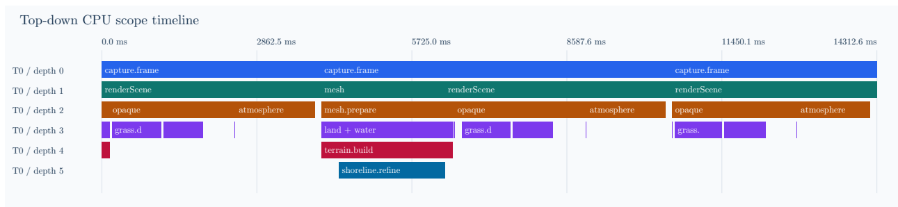
Figure 17: Top-down nested CPU scope timeline for three frozen walking frames on llvmpipe. Width represents wall time, including waits.
