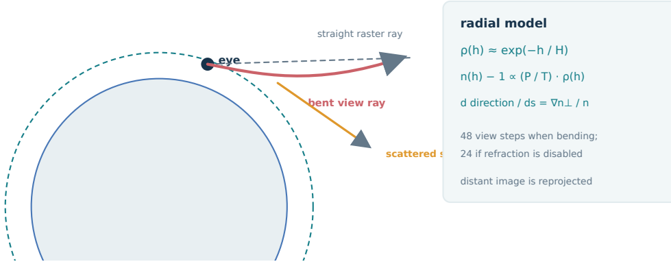
Figure 14: A refractive view ray bends through denser air while solar light contributes scattered radiance. Near terrain keeps its rasterized silhouette; only visible distant imagery is reprojected. Generated schematic.
